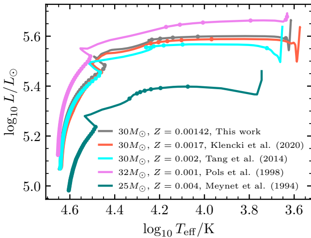
Fig. C.1. Evolution of stars with a mass of \sim 30 M_{\odot} and a metallicity of Z_{\odot}/10 computed by different research groups and codes. Dots are plotted every 10^5 years.
