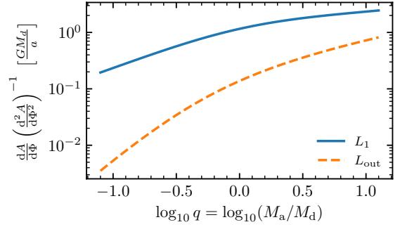
Fig. A.1. Ratio of dA/d\Phi to d^2A/d\Phi^2 at L_1 and at the outer Lagrangian point of a star expressed in units of GM_d/a .
