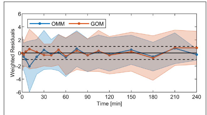
Figure 4. Mean and standard deviation of weighted residuals between the model-inferred and observed glucose levels for the oral minimal model (OMM) and the glucose-only model (GOM) identified on the same dataset.
