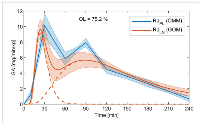
Figure 2. Example of the piecewise linear GA function Ra_{PL} used in the oral minimal model (OMM) and the log-normally based GA function Ra_{LN} used in the glucose-only model (GOM) with associated 95% confidence intervals (shaded area). The confidence intervals overlap for 75% (OL value) of the response duration of 240 min. The dashed lines indicate the two components of Ra_{LN} .
