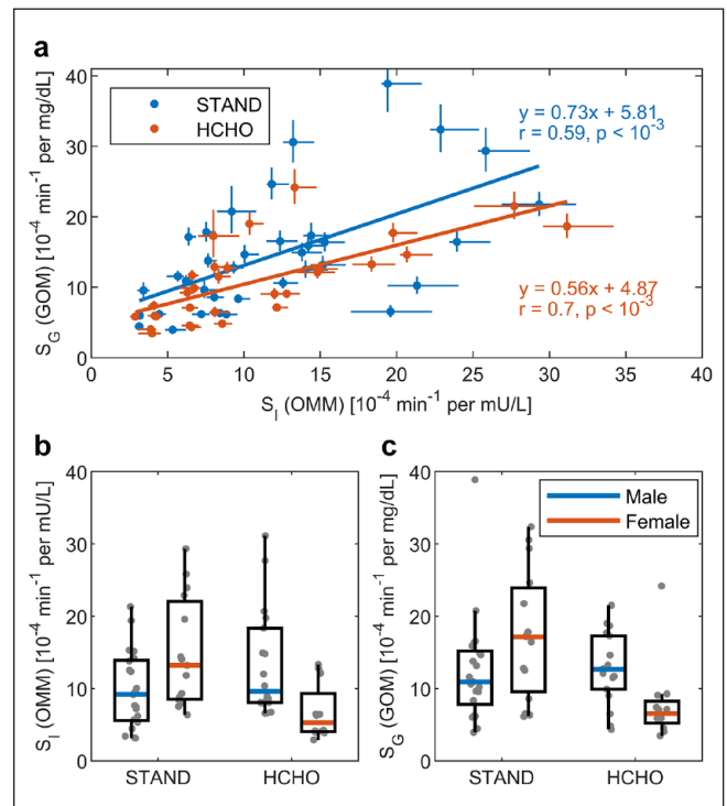
Figure 5. Results of the parameter S_G from glucose-only model (GOM) and the corresponding insulin sensitivity parameter S_I from oral minimal model (OMM). The results are compared between the meals of standard (STAND) and high carbohydrate (HCHO) composition. Plot (a) shows a correlation and linear regression analysis with the horizontal and vertical lines for each data point indicating the one-sigma range of the posterior log-normal parameter distribution. Plots (b, c) show boxplots of S_I and S_G separated by meal type and subject sex.
