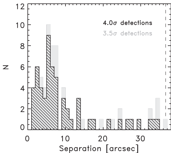
Figure 8. Histogram of the separations between the AzTEC detection and H-ATLAS targeted positions. Although a radius \theta_{500\mu\text{m}} = 36.6 arcsec (vertical dashed line) is used for our counterpart analysis, \sim 82 per cent (75 per cent) of the 4\sigma ( 3.5\sigma ) AzTEC sources are separated by \lesssim 15 arcsec off the H-ATLAS target, were the reliability of the detections is \gtrsim 98 per cent (90 per cent; see Fig. 6).
