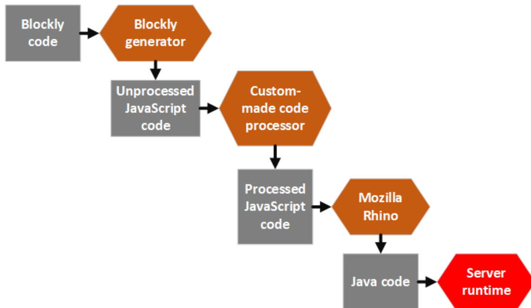
Fig. 2. The pipeline of processes used to generate, process and run code written by the players.
