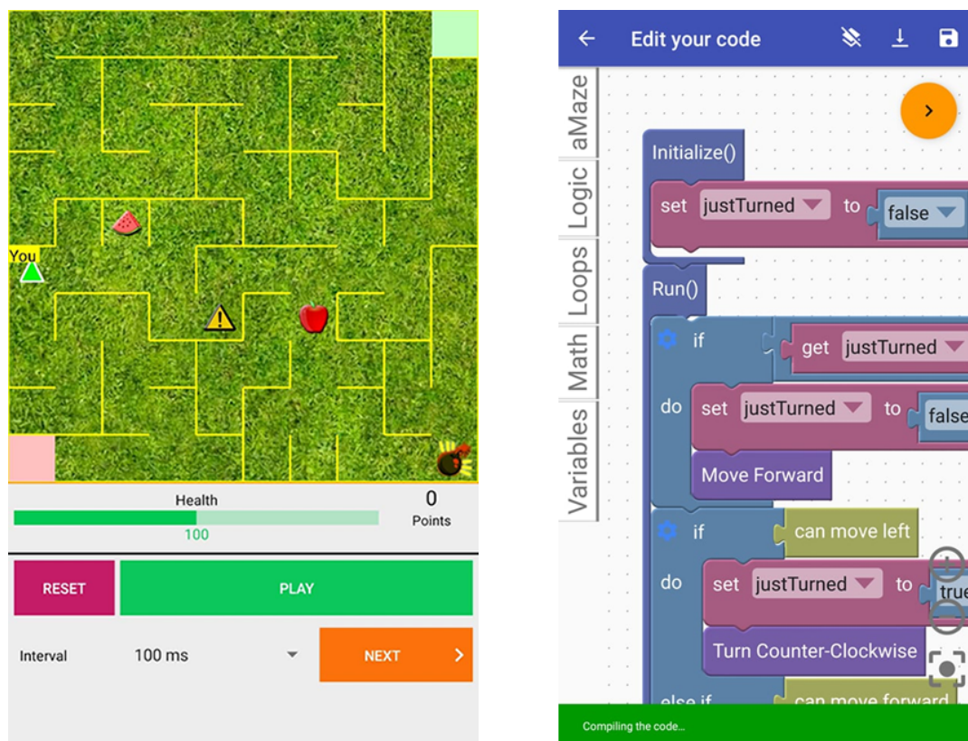
Fig. 1. A screenshot of the aMazeChallenge app: this view shows a maze which includes reward and penalty items (left side), and the Blockly-based code editor (right side).
