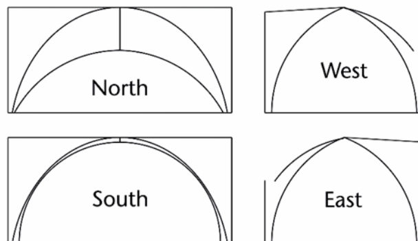
Figure 2. Tewkesbury Abbey, bay N8, design hypothesis.
