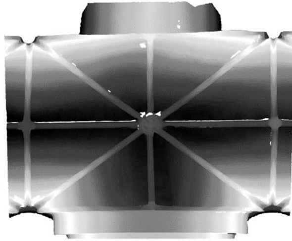
Figure 7. Tewkesbury Abbey, bay N8, height map.
