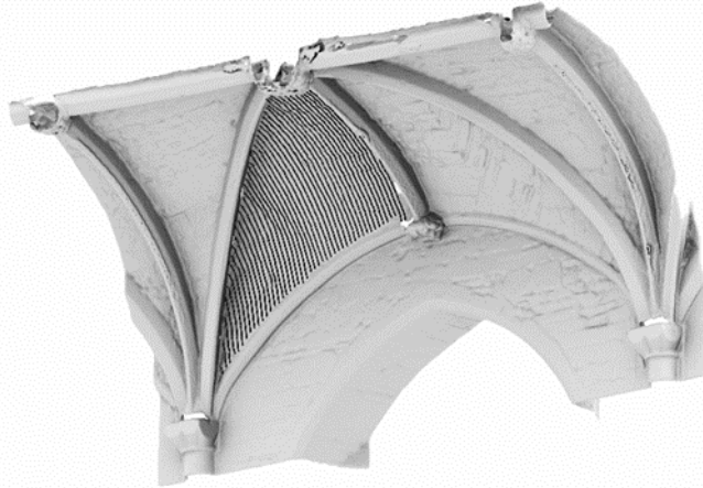
Figure 5. Tewkesbury Abbey, bay N8, contours (parallel to transverse axis) superimposed on mesh model.
