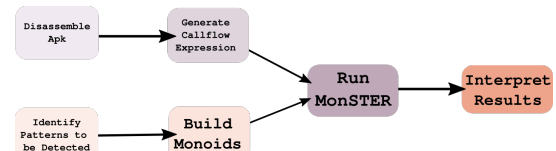
Figure 4: MonSTER workflow.
