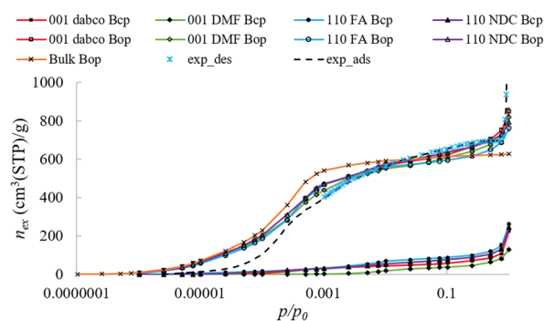
Fig. 5 N 2 adsorption isotherms at 77 K inside the simulated Bop slabs and bulk, and the experimental isotherm in rigid DUT-8 nanoparticles. Slabs are capped with: dabco, dimethylformamide (DMF), formate (FA), or H(2,6-ndc - ) (NDC).
