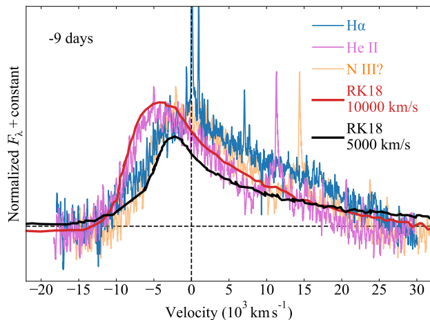
Figure 18. Velocity profiles of the strongest emission lines in the X-shooter spectrum at 9 days before peak, during the early rise/expansion phase. We show H\alpha , and the broad He II/Bowen bump for two different cases: (i) assuming that the line is dominated by He II (pink) or (ii) that it is dominated by N III (orange). Although the latter case gives a profile quite similar to H\alpha , the evolution over the next 20–30 days suggests that He II is more likely the dominant component. Overplotted are model line profiles from Roth & Kasen (2018). Assuming the blend is dominated by He II, an excellent match is found for a 10,000 \text{ km s}^{-1} outflow. H\alpha comes from slower material with velocity \lesssim 5000 \text{ km s}^{-1} .
