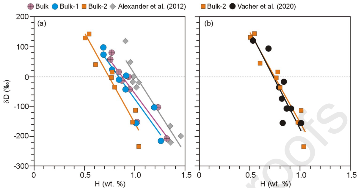
Fig. 7. Plots of wt. % H against \delta D . (a) The nine unheated CMs of subsets A and B. Compositions have been calculated using H measured over three different temperature ranges: bulk, bulk-1, and bulk-2. Correlation coefficients and equations of regression lines plotted for each dataset are: bulk ( R^2 0.82, y = -451x + 394 ); bulk-1 ( R^2 0.86, y = -470x + 396 ); bulk-2 ( R^2 0.93, y = -614x + 457 ). Bulk compositions of the same meteorites in Alexander et al. (2012) are also plotted: R^2 0.91, y = -534x + 538 . (b) Bulk-2 compositions of subset A and B samples together with the nine CM samples that were analysed by Vacher et al. (2020) after preheating to 120 °C ( R^2 0.80, y = -656x + 483 ). The dashed lines in both graphs denote 0 ‰.
