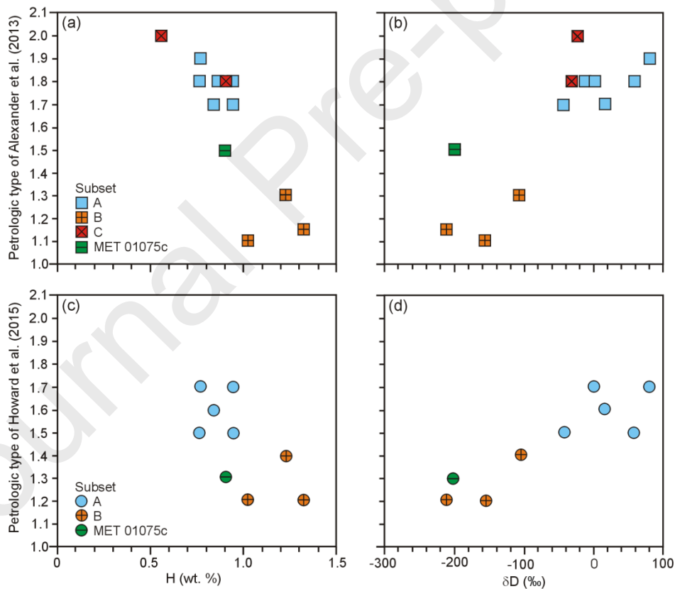
Fig. 3. Petrologic type of the analysed CMs plotted against their wt. % H and \delta D . The petrologic type of all 12 samples was determined by Alexander et al. (2013), and correlates well with wt. % H ( R^2 = 0.70 ) (a) and \delta D ( R^2 = 0.68 ) (b). The petrologic type of nine of the CMs was determined by Howard et al. (2015) and correlates poorly with wt. % H ( R^2 = 0.41 ) (c) although well with \delta D ( R^2 = 0.80 ) (d). Regression lines are not shown.
