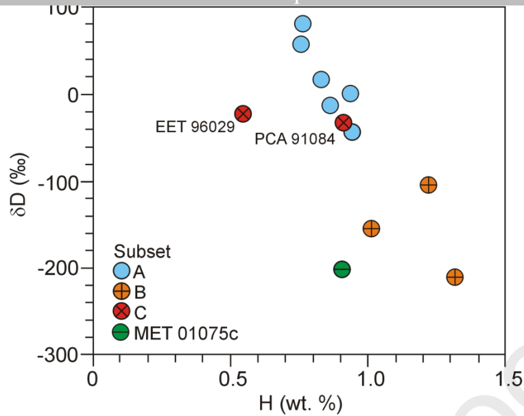
Fig. 2. Bulk hydrogen compositions of the 12 CMs analysed. The two subset C samples are labelled.
