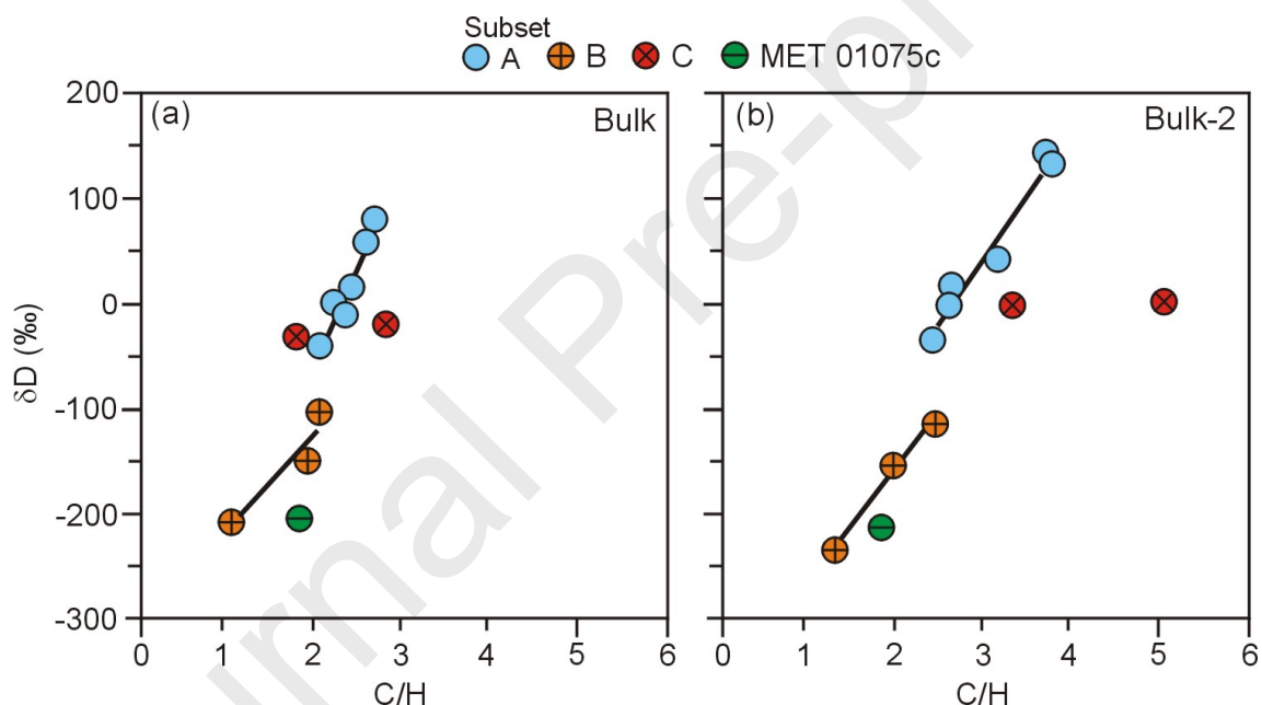
Figure 5. The bulk C/H ratio (wt. %) of the 12 CMs plotted against bulk \delta D . The wt. % H and \delta D data are from the present study whereas wt. % C for each meteorite is taken from Alexander et al. (2012) (an average of their two analyses of SCO 06043 was used) (Table 2). (a) C/H and \delta D calculated using H that was evolved over all of the pyrolysis steps. Regression lines are plotted for subsets A and B ( R^2 = 0.92 and 0.87 , respectively). (b) C/H and \delta D calculated without H that was evolved below 200 °C, which is assumed to be an adsorbed terrestrial component (termed bulk-2). Regression lines are plotted for subsets A and B ( R^2 = 0.97 and 0.99 , respectively).
