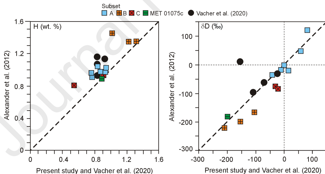
Fig. 6. Bulk wt. % H (left) and \delta D (right) of the 12 CMs that were analysed in the present study compared with the same meteorites as analysed by Alexander et al. (2012). Four of the CMs that were analysed by Vacher et al. (2020) (LON 94101, Mighei, Murchison, Murray) are likewise plotted against the same meteorites in Alexander et al. (2012). The vertical and horizontal dashed lines in the \delta D plot denote 0 ‰.
