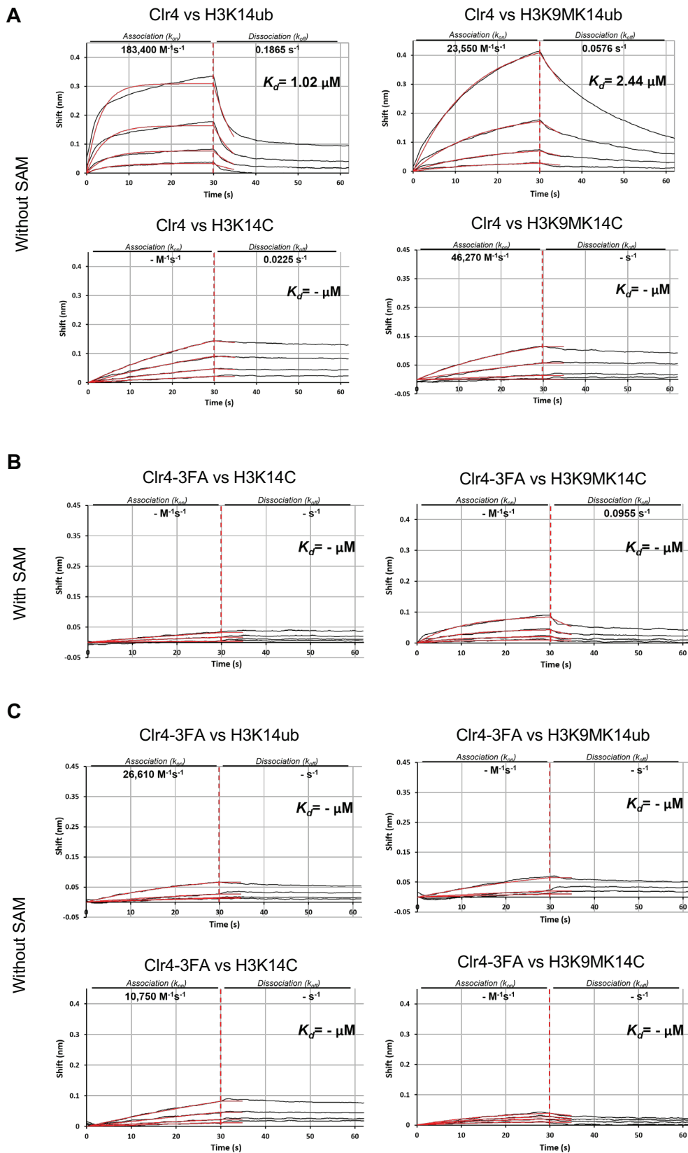
Figure S4. BLI analyses of indicated histone tail peptides with wild type Clr4-SET domain in the absence of SAM (A), with Clr4-3FA with in the presence SAM (B), and with Clr4-3FA in the absence of SAM (C). Related to Figures 3 and 4.
