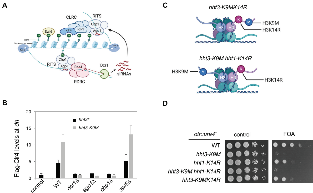
Figure S1. The requirement of CLRC for the sequestration of Clr4 by H3K9M. (A) Schematic diagram of RNAi-mediated heterochromatin assembly at DNA repeats. (B) ChIP analysis of Flag-Clr4 levels at pericentric dh repeats, normalized to act1 + . Data are presented as mean ± SD of three technical replicates. (C) Diagram of the mutations used. (D) Serial dilution analysis of indicated strains to measure the expression of otr::ura4 + . Related to Figure 2.
