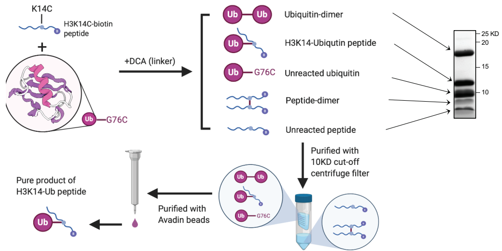
Figure S2. Diagram of the procedure used to synthesize and purify H3K14ub mimics. A SDS-PAGE of the ligation reaction production is shown on the right. Related to Figure 3.
