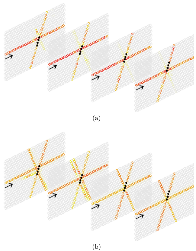
FIG. 6. Constrained ( H > 0.01 ) energy density function averaged over 50 time snapshots and 2000 individual simulations of mobile breather collisions with a stationary breather on a crystal axis at 60^\circ to the moving one. The stationary breather is at slightly different positions in each case. (a) simulation with \epsilon = 0.01 until T_{end} = 1000 . (b) simulation with \epsilon = 0.05 until T_{end} = 500 .
