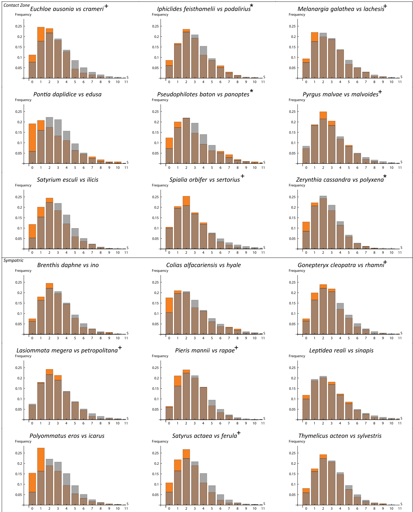
FIGURE 3 The distribution of pairwise differences, S in blocks of a fixed length of 4D sites in contact (upper box) and sympatric (lower box) pairs. The observed distribution in single-copy orthologues is shown in orange, and the expectation under a history of strict divergence (estimated from \pi and d_{ij} ), in grey. Pairs that show wider-than-expected distributions are marked with an asterisk (*), and species that show narrower-than-expected distributions are marked with a plus (+)
