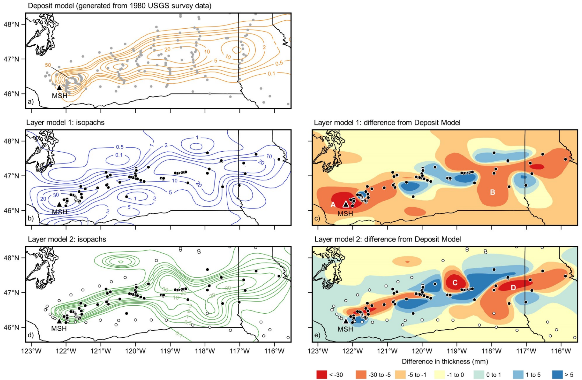
Fig. 6: A comparison of isopach maps generated using the cubic B-spline approach of Engwell et al. (2015). Panel (a) shows the Deposit Model, an isopach map generated from the 1980 survey data, with the original survey locations indicated by grey circles. Panel (b) is an isopach map of our
