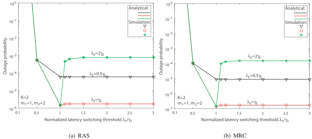
Fig. 6. Effect of the normalized \lambda_T on the outage probability of SSC-based MEC networks.
