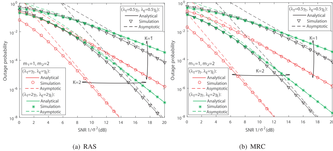
Fig. 8. Effect of number of transmit antenna on the outage probability of SSC-based MEC networks versus SNR, with several branch switching thresholds.
