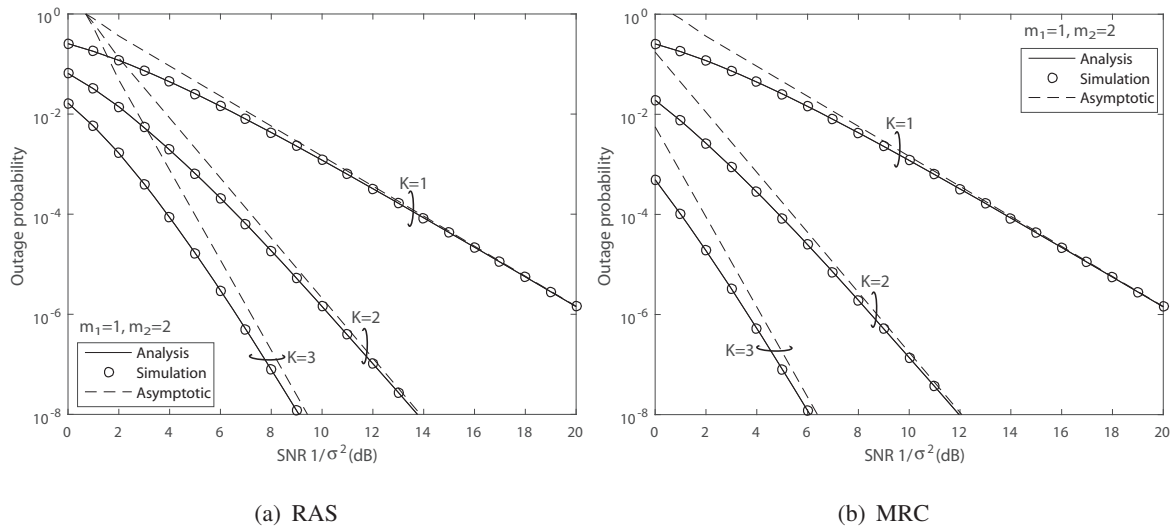
Fig. 3. Effect of number of transmit antenna on the outage probability of SC-based MEC networks versus SNR.
