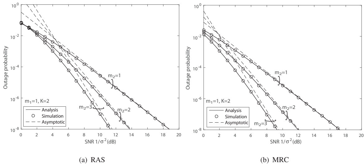
Fig. 4. Effect of Nakagami parameter on the outage probability of SC-based MEC networks versus SNR.
