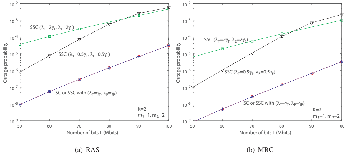
Fig. 10. Performance comparison between SC and SSC protocols with several branch switching thresholds versus L .
