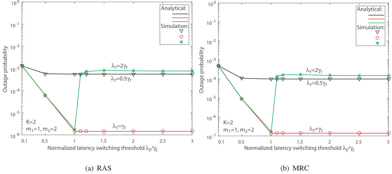
Fig. 7. Effect of the normalized \lambda_E on the outage probability of SSC-based MEC networks.
