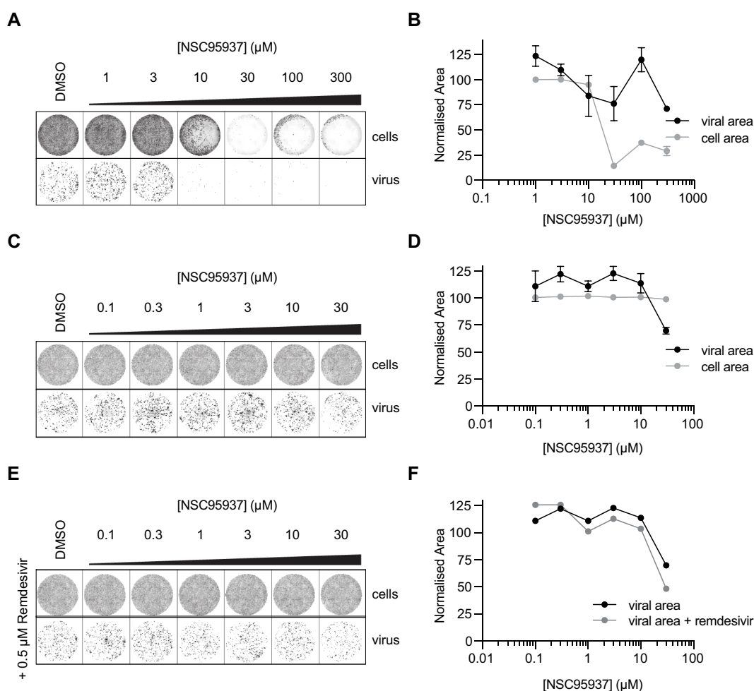
Figure 5. NSC95397 does not inhibit SARS-CoV-2 growth in VERO cells.
