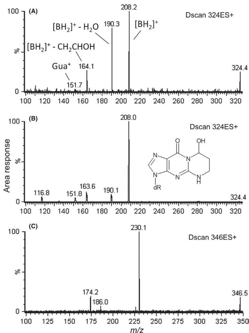
Figure 4. Results of LC/ESI(+)-MS/MS product ion scan analyses of (A) putative DNA adduct c, which corresponded to the protonated molecule [\text{M} + \text{H}]^+ = 324 , (B) an authentic standard of 8-hydroxy-PdG, and (C) putative DNA adduct d, which corresponded to the protonated molecule [\text{M} + \text{H}]^+ = 346 . Analyses were conducted at a CID of 20 eV. [\text{BH}_2]^+ is used to represent the doubly protonated base ion, [\text{M} + 2\text{H} - \text{dR}]^+ . LC/ESI (+)-MS/MS, liquid chromatography electrospray ionisation-tandem mass spectrometry in positive ionisation mode; CID, collision induced dissociation.
