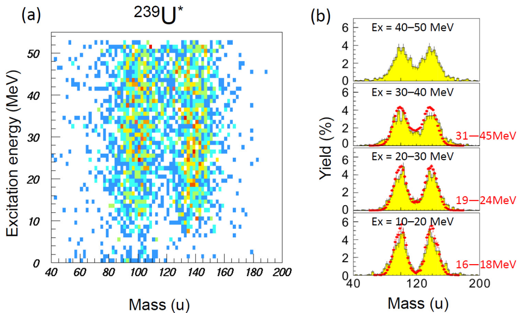
Fig. 3 (a) Fission fragment mass distribution of ^{239}\text{U}^* plotted on the mass and excitation energy. (b) Fission fragment yields obtained in the present experiment (histogram) are compared with the literature data shown by open circles. The literature data is taken from (Simutkin 2014) and the excitation energy range is marked in the right side of each panel.
