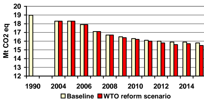
Figure 1.2 Projections of GHG emissions from Irish agriculture – Baseline and WTO scenarios
