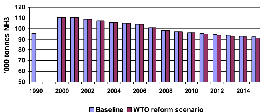
Figure 1.3 Projected ammonia emissions from agriculture – Baseline and WTO scenarios
