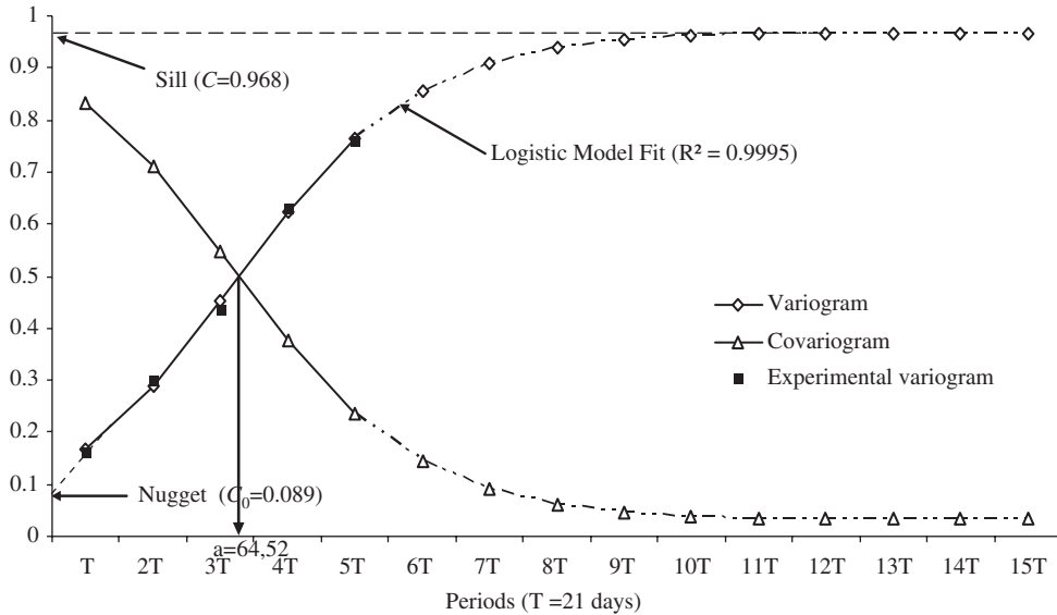
Figure 4. Descriptive variogram \gamma(\mathbf{h}) of Z scores modelled following a Logistic equation and its corresponding covariogram (i.e.: 0.968-\gamma(\mathbf{h}) ). (a) Reported on the figure corresponds to the halftime variogram.
