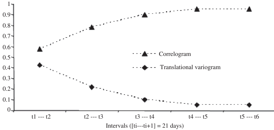
Figure 2. Translational variogram ( \gamma ) of Z scores on a period T=21 days and the corresponding correlogram (i.e., 1-\gamma ).
