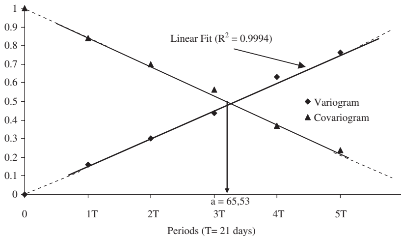
Figure 3. Descriptive variogram \gamma(h) of Z scores modelled following a linear fit and its corresponding covariogram (i.e.: 1 - \gamma(h) ). (a) reported on the figure corresponds to the halftime variogram.
