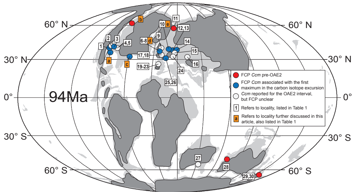
Figure 8. Compilation of the first consistent presence (FCP) of Cyclonephelium compactum – membraniphorum morphological plexus ( Ccm ) across Oceanic Anoxic Event 2. Numbers in white boxes refer to localities compiled in Table 1. Letters in orange boxes refer to the sites selected for comparison of established biozonation, high-resolution records of \delta^{13}\text{C} and the relative abundances of Ccm (Fig. 9) also compiled in Table 1. The Mollweide projected paleogeographic map for the Cenomanian–Turonian boundary interval was generated at http://www.odsn.de/odsn/services/paleomap/paleomap.html . Continental plates are in light gray. Dry land in dark gray after Scotese (2001).
