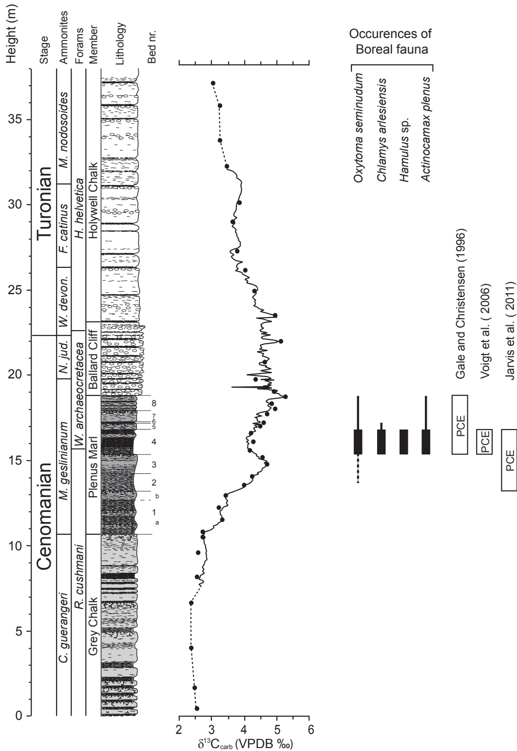
Figure 1. Biozonation, lithology, Plenus Marl beds (Jefferies, 1963) and \delta^{13}C_{carb} (low-resolution data (dots and dotted line) derived from Pearce et al., 2009; high-resolution data (solid line) derived from Paul et al., 1999) for the Cenomanian–Turonian boundary reference section at Eastbourne, combined with occurrences of Boreal fauna (Gale and Christensen, 1996). On the right side the ranges of the different definitions for the Plenus Cold Event are indicated.
