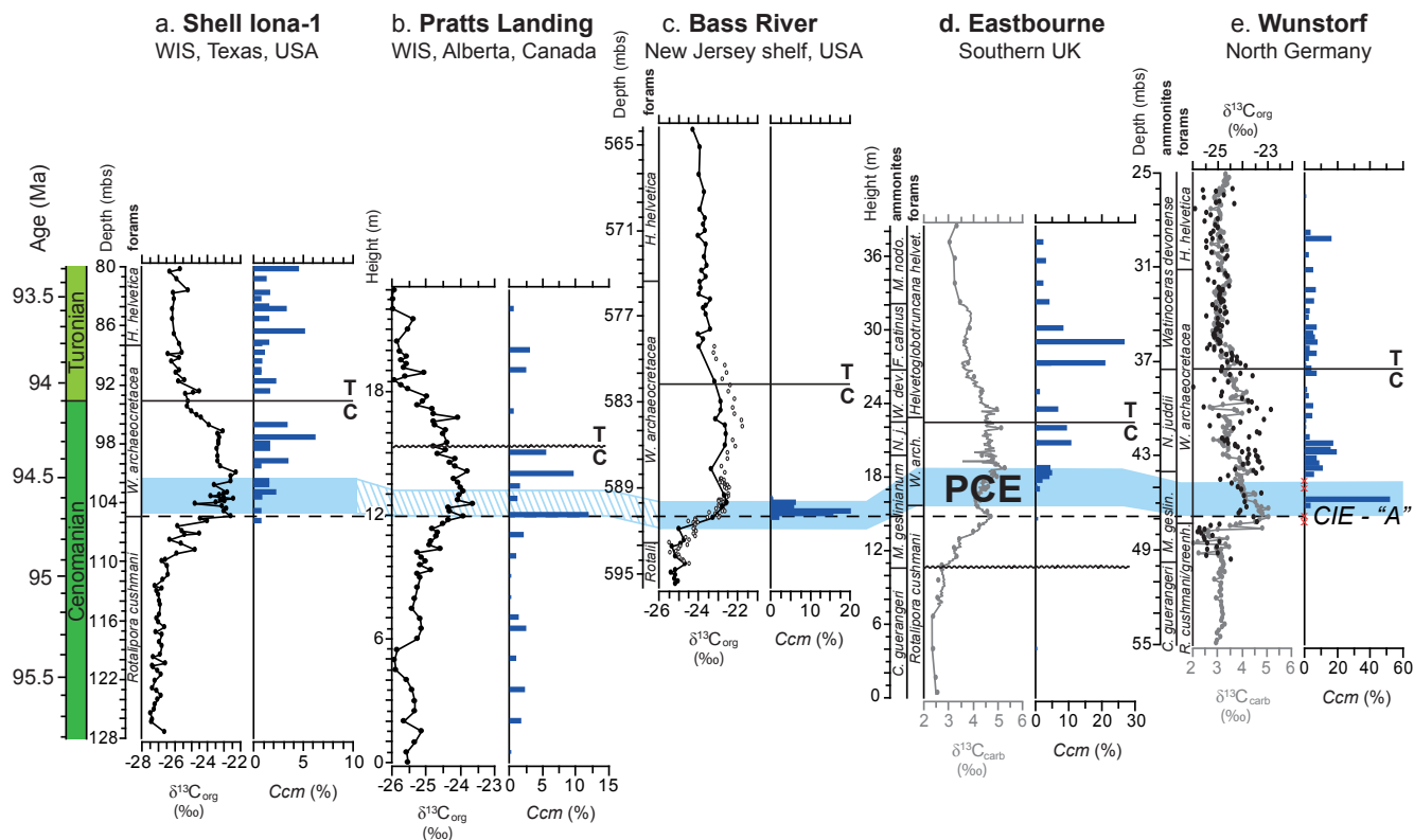
Figure 9. Overview of \delta^{13}\text{C}_{\text{org}} and/or \delta^{13}\text{C}_{\text{carb}} , abundances of Cyclonephelium compactum – membraniphorum morphological plexus ( Ccm ) and foraminiferal and/or ammonite zonation for the studied sections. (a) Shell Iona-1 core (Eldrett et al., 2014). (b) Pratts Landing (this study). (c) Bass River (van Helmond et al., 2014a); open symbols are \delta^{13}\text{C}_{\text{org}} derived from Bowman and Bralower (2005). (d) Eastbourne (Pearce et al., 2009); high-resolution \delta^{13}\text{C}_{\text{carb}} data derived from Paul et al. (1999). (e) Wunstorf – relative abundances of Ccm from van Helmond et al. (2015), \delta^{13}\text{C}_{\text{org}} from Du Vivier et al. (2014) and \delta^{13}\text{C}_{\text{carb}} from Voigt et al. (2008); a red cross marks a barren sample. Age is from the astronomically tuned age model for the Shell Iona-1 core (Eldrett et al., 2015). Dashed line represents the first maximum in the carbon isotope excursion, point “A” (cf. Voigt et al., 2008). Solid lines represent the Cenomanian–Turonian boundary. The blue shaded area represents the Plenian Cold Event according to its original definition (Gale and Christensen, 1996), the cooling in reconstructed sea surface temperatures at Bass River and Wunstorf (van Helmond et al., 2014a, 2015), and the (re)oxygenation of bottom waters in the Shell Iona-1 core (Eldrett et al., 2014). Note: the sections are plotted using different depth scales.
