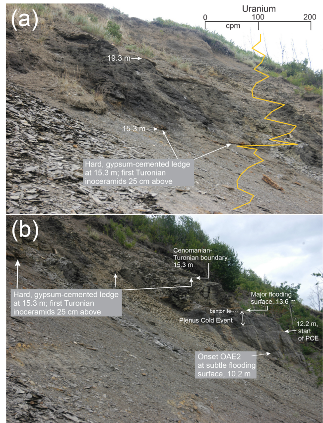
Figure 5. Field photographs of the Pratts Landing site. Photograph (a) shows an overview of upper part of the section showing resistant, gypsum-cemented ledge that marks a sharp erosional boundary between two claystone units. Immediately above the boundary there is a large increase in the uranium content of the sediment. The early Turonian inoceramid bivalves Mytiloides goppelnensis and Mytiloides kossmati appear 25 cm above the erosion surface. Photograph (b) shows an overview of the lower part of the section showing highly bioturbated silty sandstone of Kaskapau allomember 6, sharply overlain, at a major flooding surface (13.6 m level) by thinly bedded claystones. Rocks embracing the Plenus Cold Event are represented by a 1.4 m thick, shallowing (sandier)-upward succession bounded above by a major flooding surface. The Cenomanian–Turonian boundary, marked by a resistant ledge, lies at the 15.3 m level. Note that all of Kaskapau allomember 7 is absent at the erosion surface marking the Cenomanian–Turonian boundary, as illustrated in Fig. 3.
