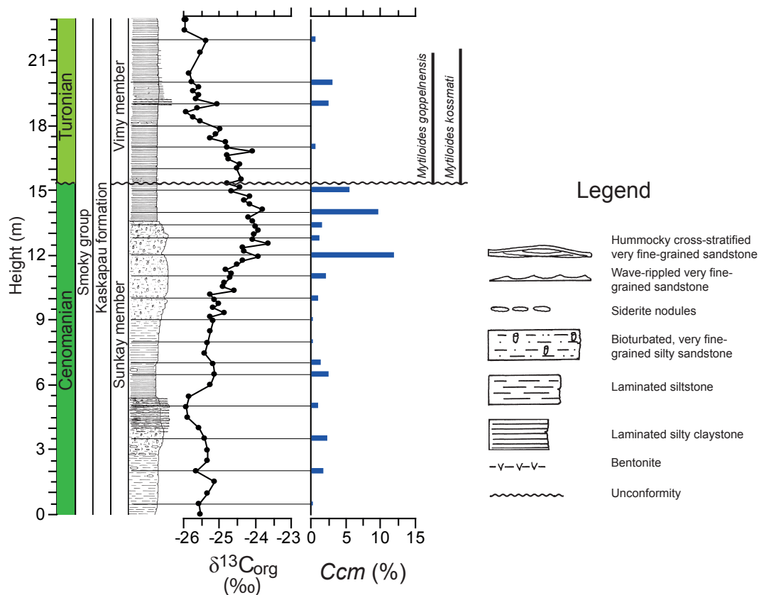
Figure 6. Lithostratigraphy, detailed lithological log, \delta^{13}\text{C}_{\text{org}} , abundances of Cyclonephelium compactum – membraniphorum morphological plexus ( Ccm ) and inoceramid bivalve stratigraphy for Pratts Landing. Sample intervals for palynology are indicated by horizontal black lines.
