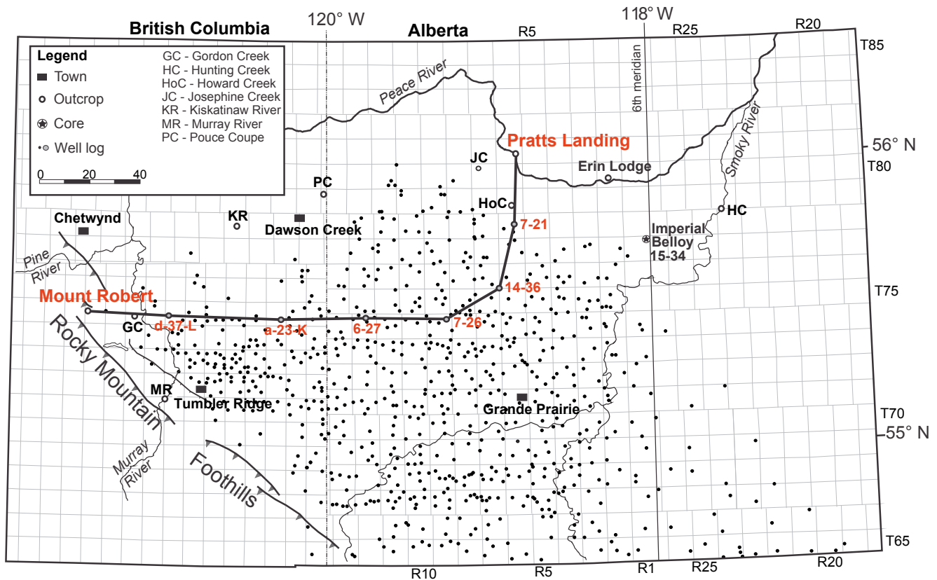
Figure 2. Map of northwestern Alberta and adjacent British Columbia showing distribution of well logs, cores and outcrops used to establish the regional stratigraphic framework that forms the basis for the present study. Outcrop sections at Mount Robert in the west and Pratts Landing in the east are correlated via wireline well logs (gamma ray and resistivity pairs).
