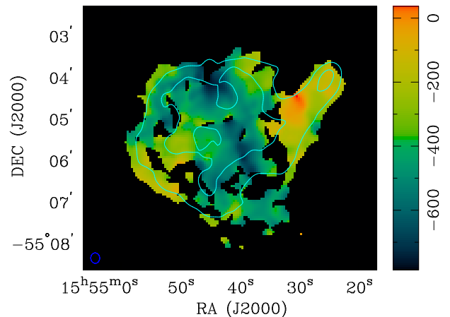
FIG. 6.— RM map of the Snail. Contours are from the 6 cm image of the PWN at levels of 4 and 8 mJy beam -1 . The color map represents the RM distribution of the Snail in units of rad m -2 . The restoring beam is shown at the lower left corner.
