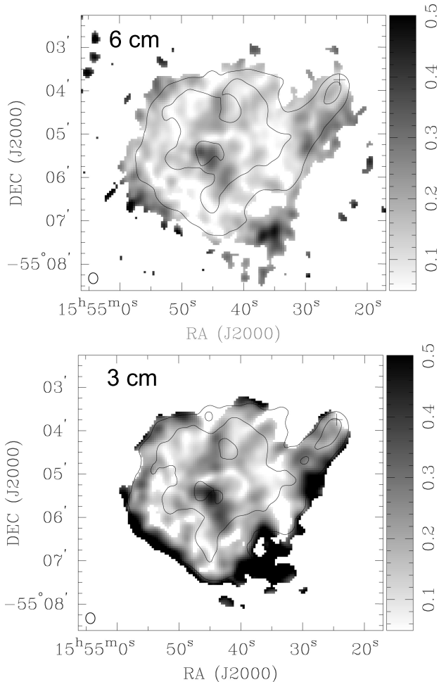
FIG. 5.— Fractional polarization of the Snail at 6 and 3 cm. The contours are from the total intensity map of 4 and 8 mJy beam -1 at 6 cm, and 1.5 and 4.5 mJy beam -1 at 3 cm. FWHM of the beams are shown in the lower left. The crosses mark the position of the X-ray point source. Note that the polarization at the edge is likely overestimated (see Section 3.3).
