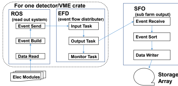
Figure 38: The data flow software. Details can be found in Sec 7.5.
