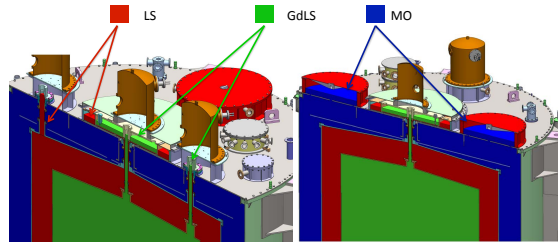
Figure 11: Orthogonal slices through the top of an AD showing the GdLS (green), LS (red), and MO (blue) overflow tanks and calibration tubes.
