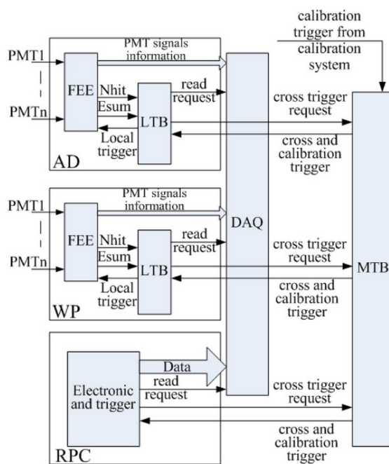
Figure 36: Layout of the trigger system. In each PMT-based detector system (AD, IWS, or OWS), the number of PMTs over the threshold (Nhit) and the analog sum of PMT signals (Esum) are sent to the Local Trigger Board (LTB), which will generate a local trigger once the prescribed trigger conditions are met. DAQ software reads PMT signal information from the FEEs and trigger information from the LTB upon receiving a trigger. The LTB in one subsystem can also initiate a trigger in a different subsystem by sending a trigger request to the Master Trigger Board (MTB), which can send trigger requests (cross triggers and calibration triggers) to all of the subsystems in the same experimental hall. The RPC trigger board differs in detail, but can also send and receive triggers to the MTB.
