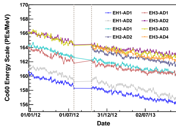
Figure 46: The energy scale from ^{60}\text{Co} calibrations at the detector center is monitored over time. The 2012 shutdown period occurs between the two grey dashed lines.
