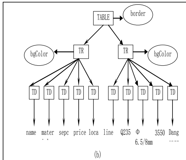
Figure3 the DOM of HTML
