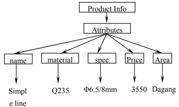
Figure4 Semantic DOM tree
