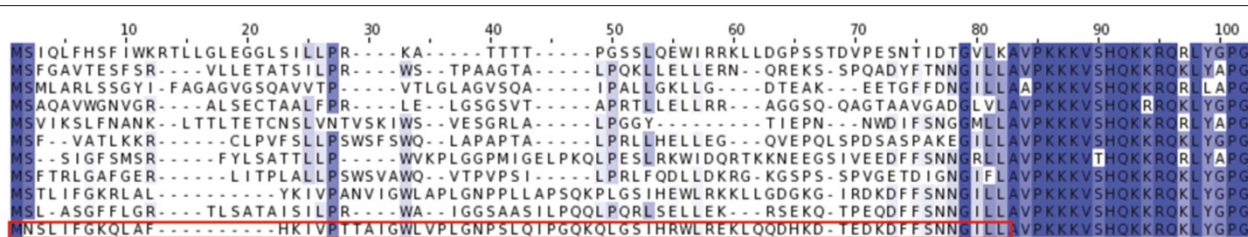
Figure 7 MSA of MrpL32 and its orthologs in 11 yeast species. Multiple sequence alignment of MrpL32 in S.cerevisiae and its orthologs in 10 other yeast species. The red boxed region shows MTS of MrpL32 . The conserved positions are colored by Jalview.
