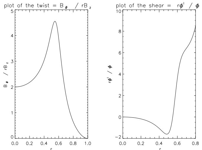
Fig. 1. The twist and shear of Equilibrium 1 .
