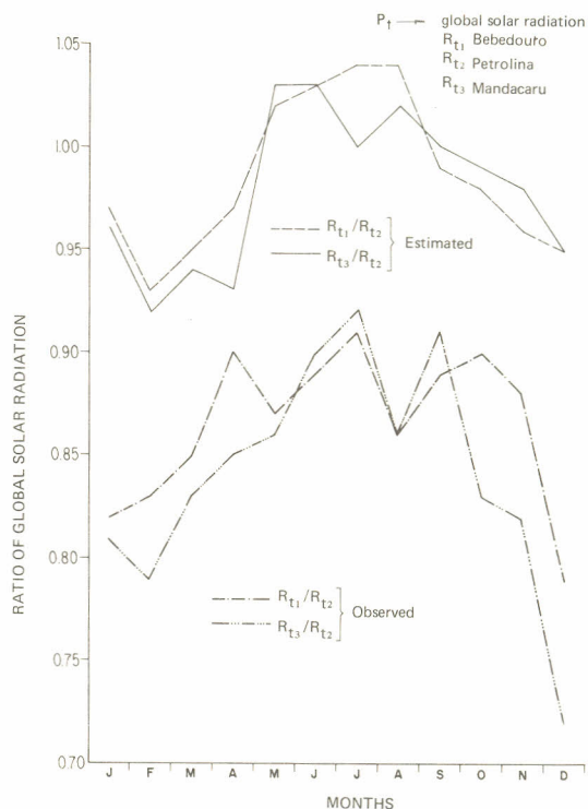
FIG. 2. Comparison of ratio of global solar radiation recorded at Bebedouro, Mandacaru to Petrolina (observed and estimated).
