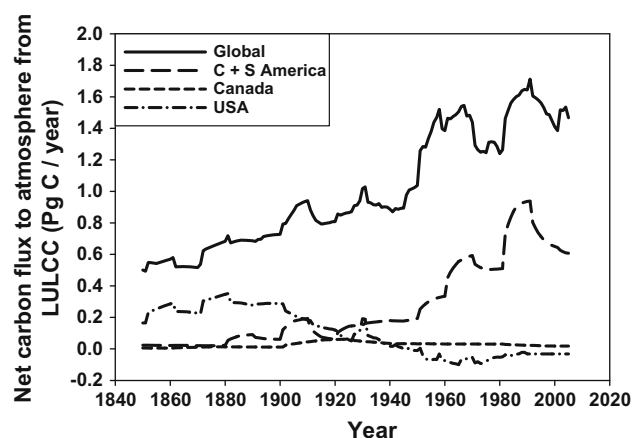
Fig. 3 Total net annual flux of carbon (Pg C/year) to the atmosphere from land use and land cover change (LULCC) globally and in Central and South America (C + S Am), Canada and the USA (data from Houghton 2008)
