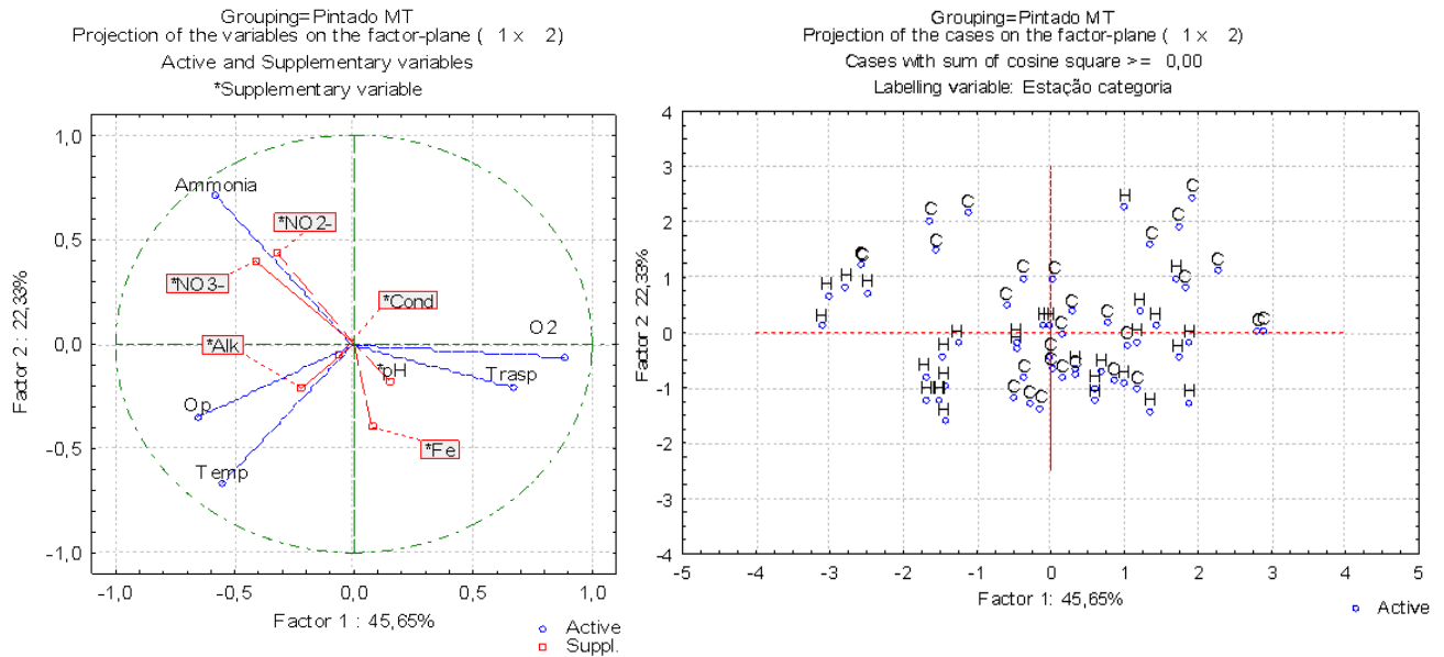
Figure 2 - Principal Components Analysis (PCA) of water quality parameters from intensive culture of hybrid surubim. O 2 = Dissolved Oxygen; Op= Orthophosphate; Trasp= Transparency; Cond= Eletrical Conductivity; Temp= Temperature; Alk= Alkalinity; Fe = Iron; C = Cold season; H = Hot season.
