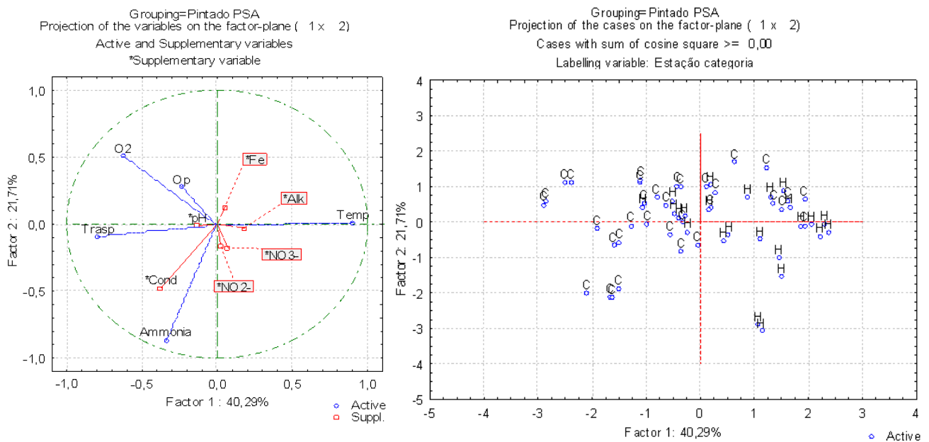
Figure 1 - Principal Components Analysis (PCA) of water quality parameters from semi-intensive culture of hybrid surubim. O 2 = Dissolved Oxygen; Op= Orthophosphate; Trasp= Transparency; Cond= Electrical Conductivity; Temp= Temperature; Alk= Alkalinity; Fe= Iron; C = Cold season; H = Hot season.
