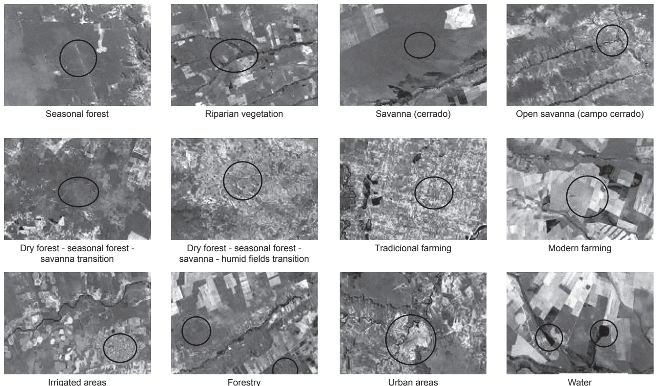
Figure 3. Land-use/land-cover classes mapped in Western Bahia, Brazil.
