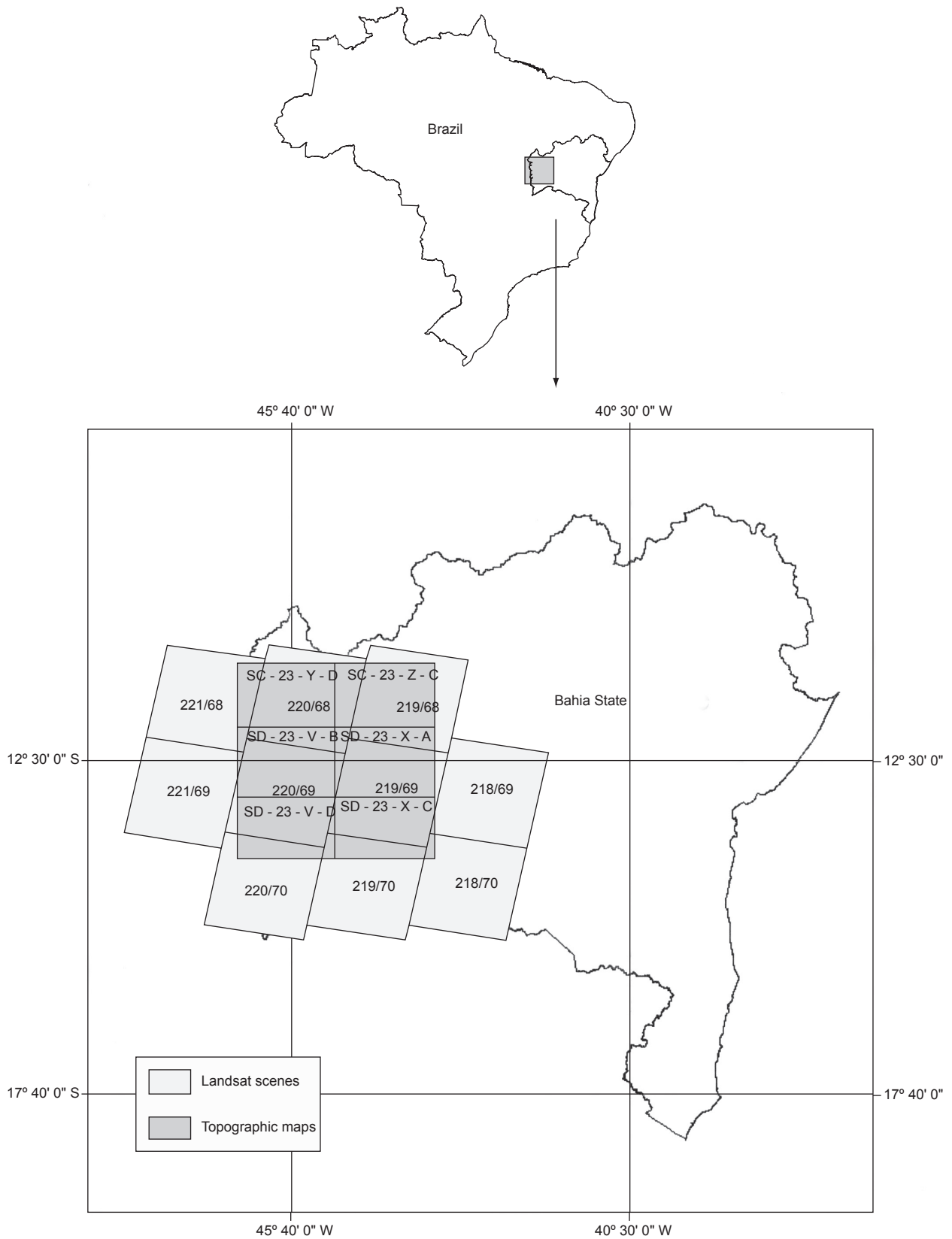
Figure 1. Topographic maps and Landsat scenes covering the study area in Western Bahia, Brazil.
