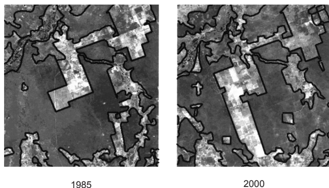
Figure 2. Land-use/land-cover vectors overlaid to subsets of Landsat mosaics from 1985 and 2000.
