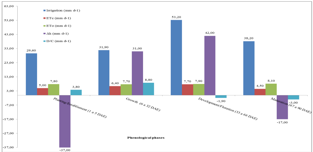
Figure 4. Irrigation (I), crop (ETc) and reference (ET 0 ) evapotranspiration, soil water storage (Δh) and soil drainage rates (D/C) daily averages for the different sesame BRS 196 CNPA G4 phenological phases. Barbalha, CE, Brazil, 2012.
