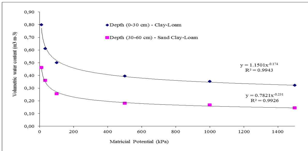
Figure 3. Soil water retention curves at 0-30 and 30-60 cm depths. Barbalha. CE. Brazil. 2012.
