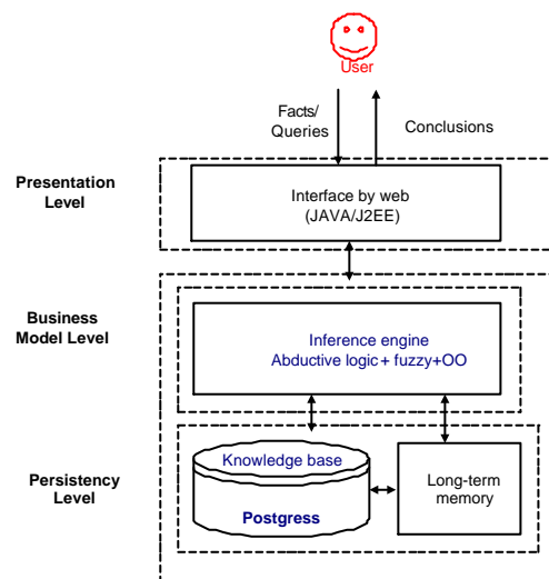
Fig. 1 An object-oriented framework for diagnosis.
