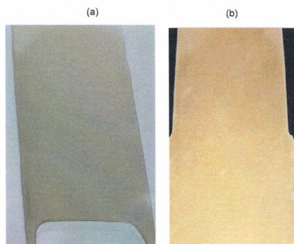
Fig 2: (a) Latex, (b) rubber/CNCs nanocomposite
