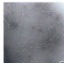
Figure 1: TEM of CNCs at 180 min
