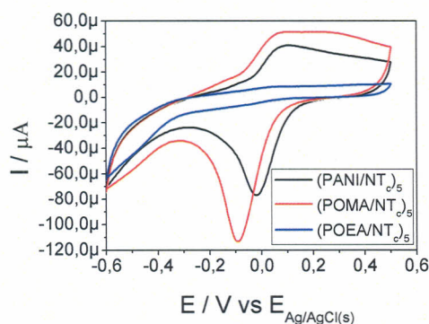
Figure 1: Cyclic voltammograms of the LbL systems employed.
