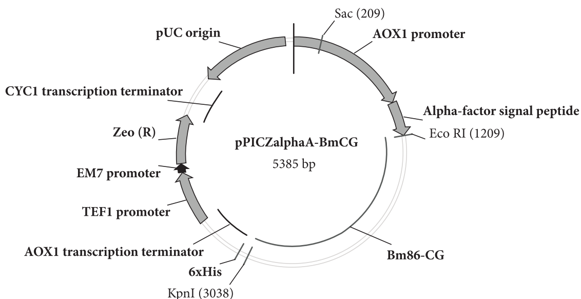
Figure 1. Map of plasmid vector pPICZ \alpha A-Bm86-CG used to transform P. pastoris expression system. The map was created with Vector NTI 8 software; 5'AOX1 promoter: promoter strongly induced by methanol; Sac I: enzyme used to linearize the plasmid before transformation in P. pastoris ; Alpha-factor: sequence corresponding of secreted peptide of rBm86-CG; EcoR I: recognition sequencing of the enzyme used for cloning of 5' region; Bm86-CG: bm86-CG sequence inserted in plasmid; Kpn I: recognition sequence of the enzyme used for cloning the 3' region; 3'AOX1 Termination: sequence that determines the end of the transcript; Zeo(R): Zeocin™ resistance gene allowing selection of transformants in Pichia ; pUC origin: Replication origin for Escherichia coli .
