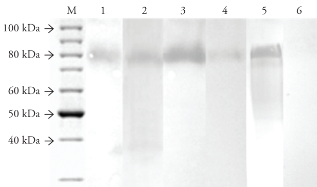
Figure 3. Western blot of rBm86-CG expressed in clone Mut + . Lanes 1: anti-Gavac™ serum; 2: anti-TickGard PLUS serum; 3: anti-larval extract serum; 4: anti-rBm86-CG serum; 5: larval extract as antigen recognized by bovine serum immunized with rBm86-CG; 6: Negative control. M: BenchMark™ Protein Ladder standards for SDS-polyacrylamide gel electrophoresis ranging in molecular weight from 10 to 220 kDa.
