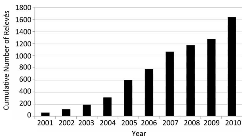
Fig. 3: Cumulative increase in RAPELD relevés in the PPBio data repository with time.
