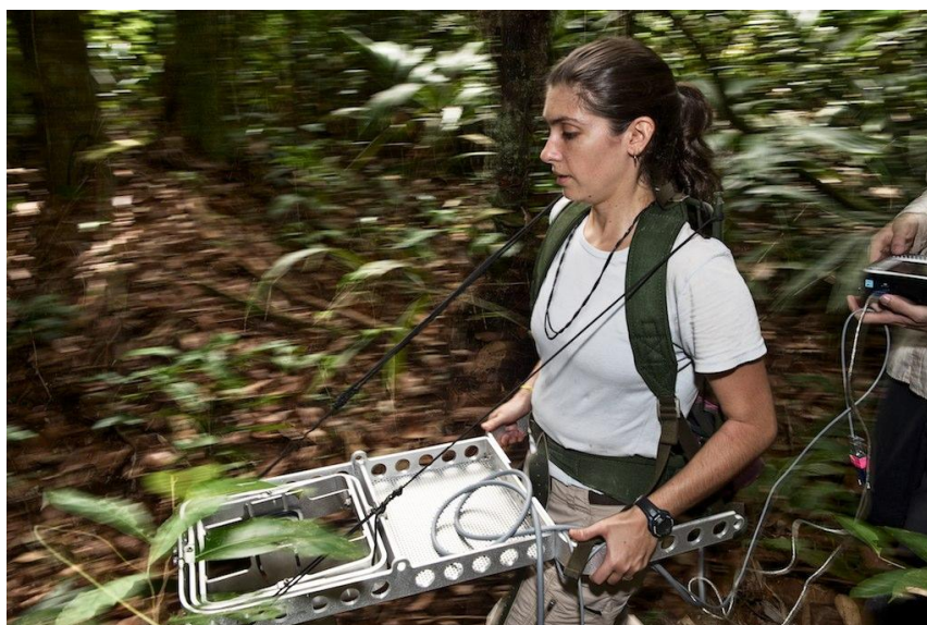
Fig. 4: Ground LIDAR survey used for calibration of relevés based on remote sensing technology (Photo: J. Bryant; http://www.envirofoto.com ).
