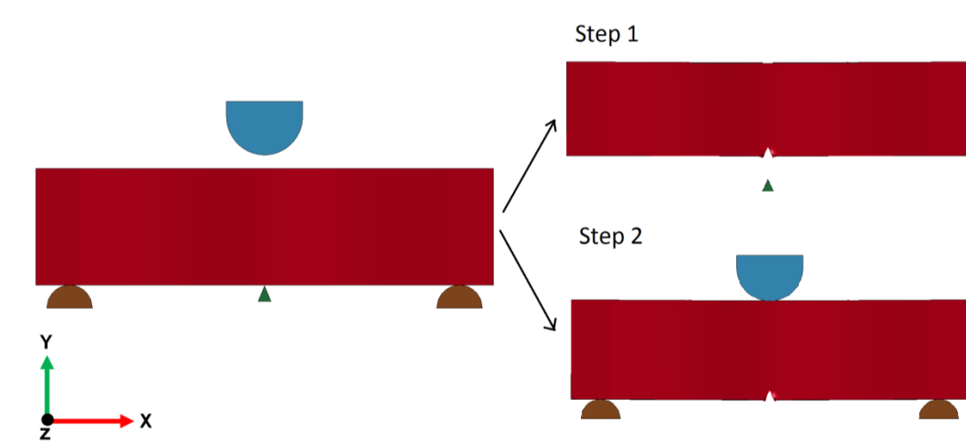
Figure 4.25 Geometry of the full simulation process
