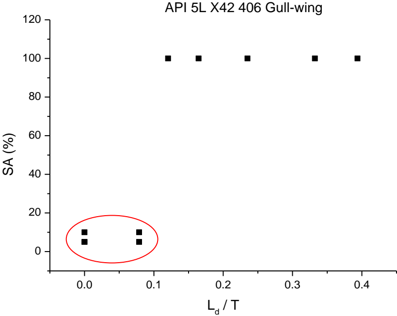
Figure 4.18 SA% vs. L d / T for X42 406 specimens
