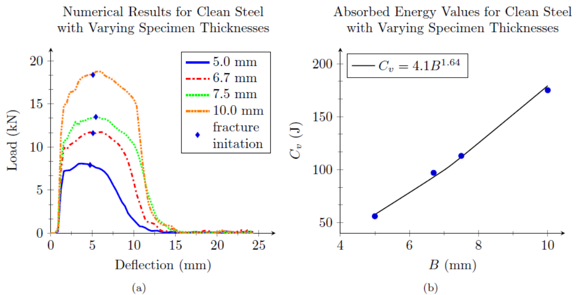
Figure 6.8 (a) Load-deflection curves for clean steel (b) Absorbed energy /specimen thickness relationship for clean steel
