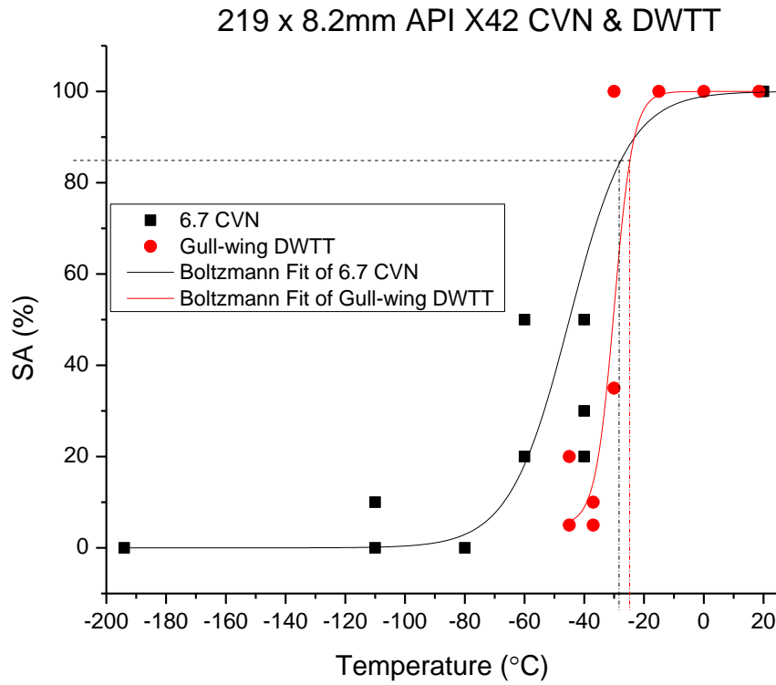
Figure 7.8 DWTT and CVN SA% vs. temperature, 406 x 12.7mm X42 line pipe
