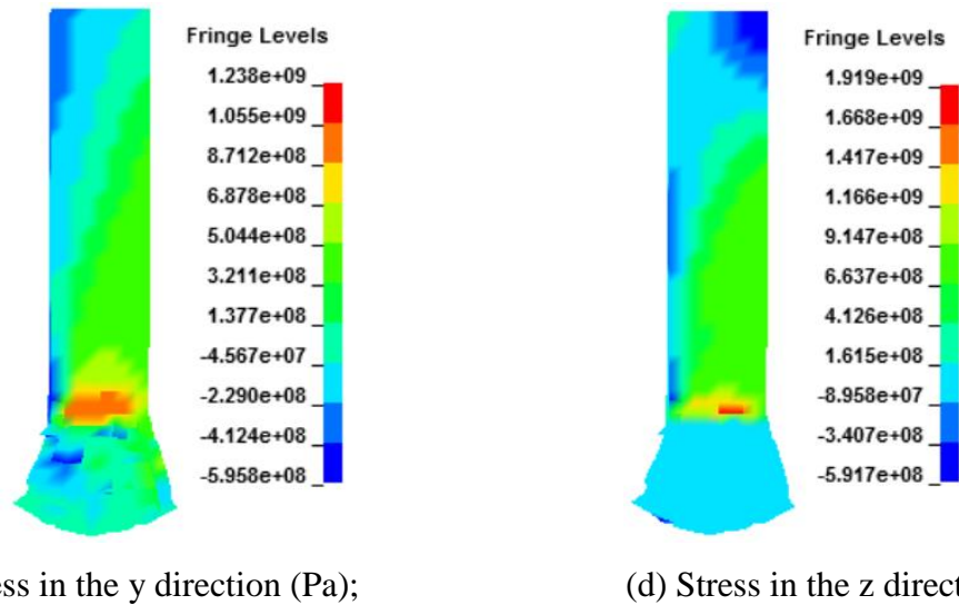
Figure 4.29 Contour results of stresses near the notch before fracture initiation ( t=2.2\text{ms} )
