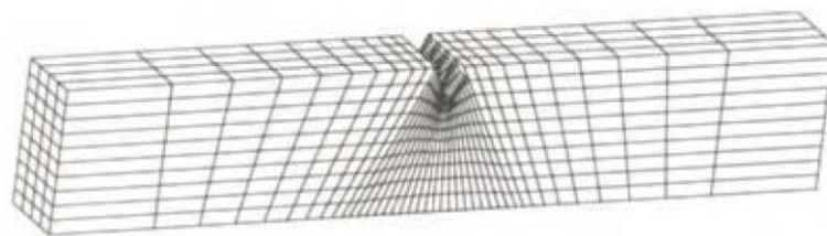
Figure 2.38 Charpy specimen and finite element half-thickness mesh [70]
