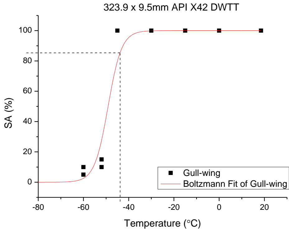
Figure 7.6 DWTT SA% vs. temperature, 323.9 x 9.5mm X42 line pipe
