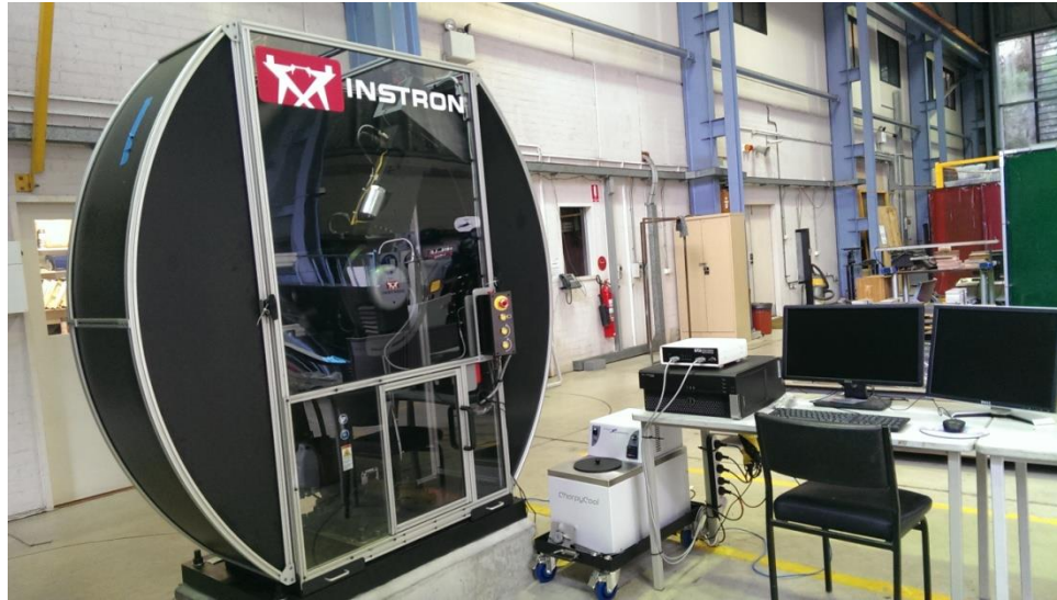
Figure 3.7 Instron MPX7500 Charpy impact test machine and cooling chamber
