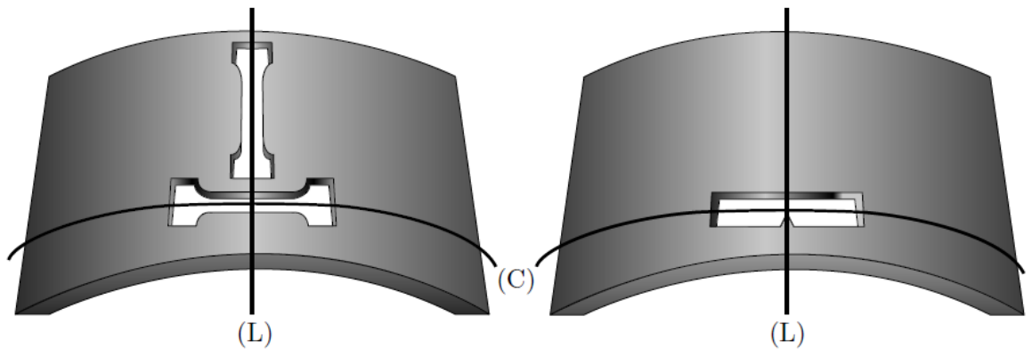
Figure 6.1 Depiction of the extraction of tensile and Charpy specimens in the longitudinal (L) and circumferential (C) orientations
