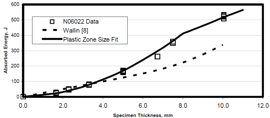
Figure 2.26 Impact energy vs. specimen thickness for N06022 [59]
