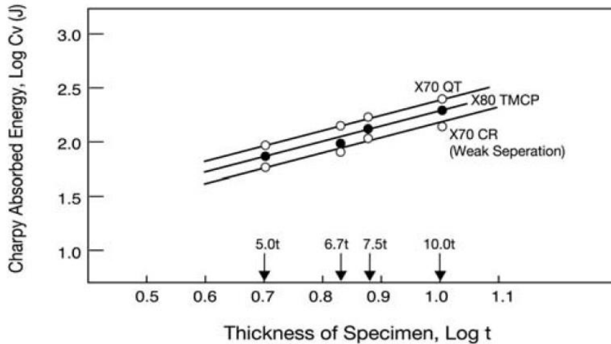
Figure 2.36 Effect of specimen thickness on upper shelf energy per unit ligament [49]
