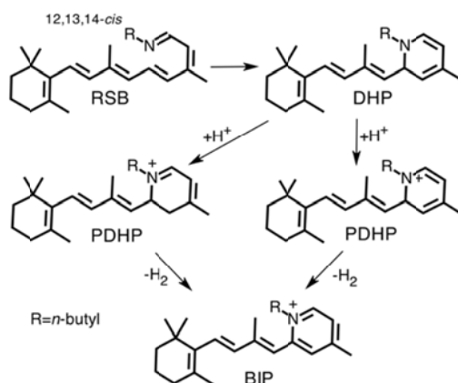
Scheme 2: Successive transformation of RSB to dihydropyridine (DHP), protonated dihydropyridine (PDHP), and N-n -butyl-2-(β-ionylidene)-4-methylpyridinium (BIP).
