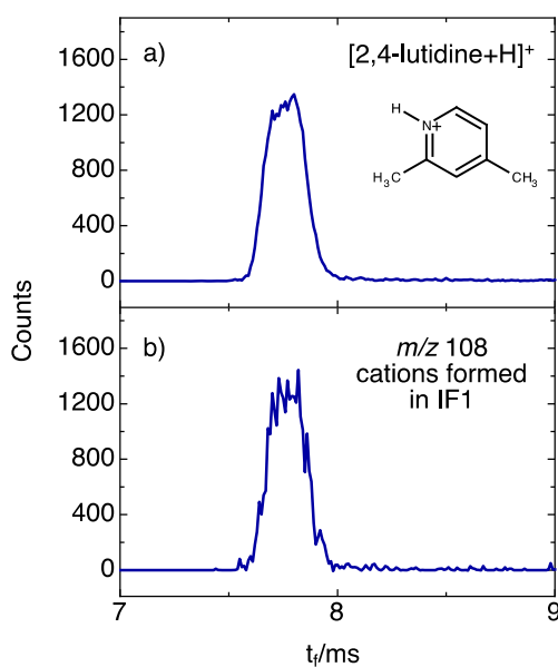
Figure 3: Arrival time distributions ( P = 6.2 Torr, N_2 buffer gas) for: a) electrosprayed reference protonated 2,4-lutidine; and b) m/z = 108 ions formed through collisional activation of electrosprayed ions in IF1.
