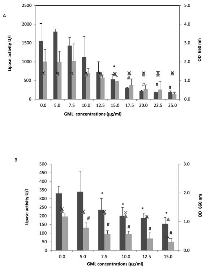
FIGURE 4. Effect of increasing concentrations of GML on bacterial cell viability and lipase production. (A) Glycerol monolaurate proved nontoxic to S. aureus 020 and S. aureus 134 up to 25 µg/mL GML and inhibited the bacterial lipases in a dose-dependent manner. * and # indicate significant differences ( P < 0.05 ) in the lipase production in the presence of GML by S. aureus 020 and S. aureus 134, respectively, compared with their lipase production in the absence of GML. ■ S. aureus 020 ■ S. aureus 134 ▲ S. aureus 020 growth × S. aureus 134 growth. (B) Glycerol monolaurate was nontoxic to S. epidermidis 001 and 024 up to a concentration of 15 µg/mL. Glycerol monolaurate inhibited the bacterial lipases in a dose-dependent manner. * and # show significant differences ( P < 0.05 ) in the lipase production in the presence of GML by S. epidermidis 001 and S. epidermidis 024, respectively, compared with their lipase production in the absence of GML. ■ S. epidermidis 001 ■ S. epidermidis 024 ▲ S. epidermidis 001 growth × S. epidermidis 024 growth.
