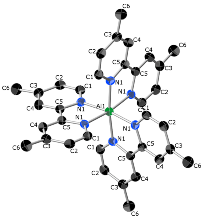
Figure 3. Crystal structure of the [\text{Al}(\text{Me-bpy})_3] complex 2 . Thermal ellipsoids drawn at the 50% probability level. Hydrogen atoms have been omitted for clarity.
