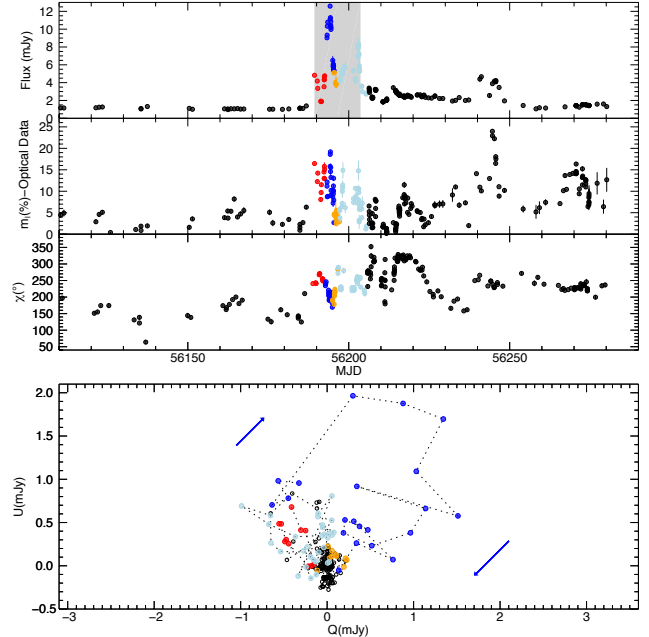
FIG. 12.— The upper panel displays, from top to bottom, the light-curve, degree and time evolution of polarization, and EVPA at optical frequencies. Each colored mark corresponds to the period over which we plot the U and Q Stokes parameters in the lower panel. Blue points mark a clockwise rotation cycle that occurs in coincidence with the total intensity peak. The gray vertical stripe indicates the time range of the main gamma-ray flare.
