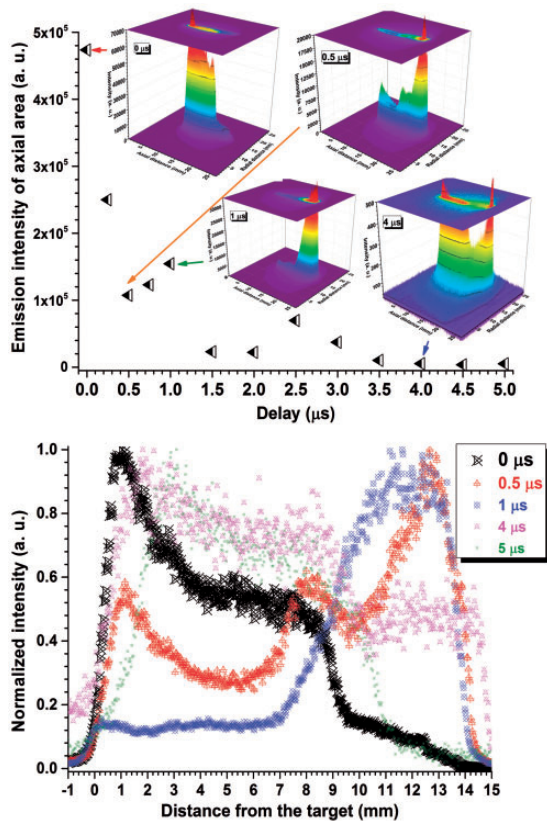
Figure 5. (Top figure) Emission intensity of axial plasma area at atmospheric pressure. Inset plots show four images at different delay times; (bottom figure) normalized axial intensity profiles from the ICCD images of the plasma at atmospheric pressure as a function of time delay.
