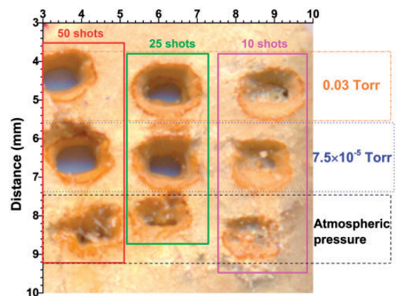
Figure 6. Photograph showing the swine muscle tissue surface characteristics after irradiating by 10, 25, and 50 laser pulses in vacuum ( 7.5 \times 10^{-5} and 0.03 \text{ Torr} ) and atmospheric pressure.
