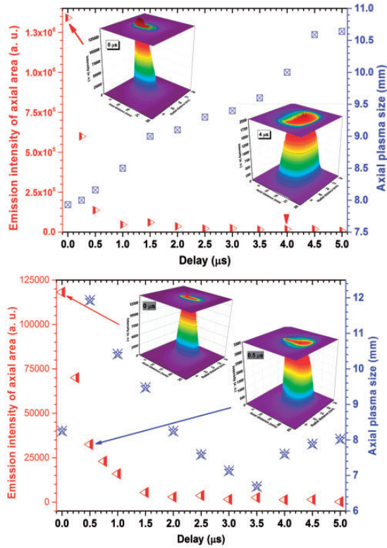
Figure 2. Emission intensity of axial area and axial plasma size (FWHM) at: 7.5 \times 10^{-5} Torr (top figure); 2.8 \times 10^{-2} Torr (bottom figure); as a function of time delay from the beginning of the laser pulse. Inset plots show images at different delays.
