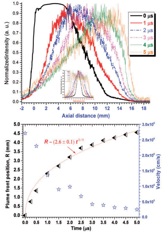
Figure 3. (Top panel) Normalized axial intensity profiles from the ICCD images of the plasma in vacuum ( P_{\text{air}} = 7.5 \times 10^{-5} Torr) as a function of time delay. The inset shows the normalized radial intensity profiles; (bottom panel) distance–time ( R-t ) plot and velocities obtained from the ICCD images of the plasma in vacuum ( P_{\text{air}} = 7.5 \times 10^{-5} Torr) are given along with the fit to a shock wave model.
