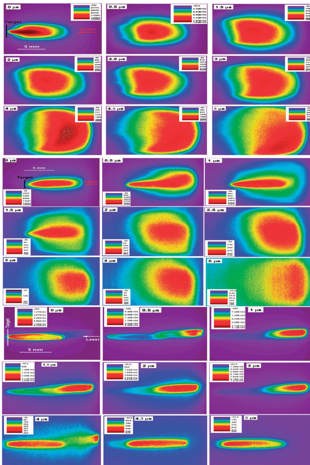
Figure 1. Time-resolved ICCD images of swine tissue at different background pressures: 7.5 \times 10^{-5} Torr (top row); 2.8 \times 10^{-2} Torr (middle row); atmospheric pressure (bottom row). The exposure time was t_w = 100 ns. The timings in the images represent the time after the beginning of the laser pulse. All of the images are normalized to their maximum intensity being the pseudo-color scale indicated for each figure.
