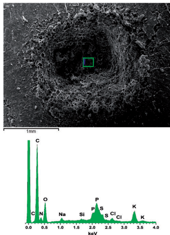
Figure 8. Scanning electron micrograph showing sample ablated surface characteristics (75 Torr) and its corresponding EDX microanalysis spectrum for the indicated area.
