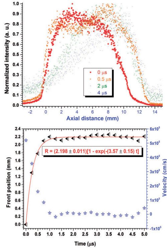
Figure 4. (Top figure) Normalized axial intensity profiles from the ICCD images of the plasma in medium vacuum ( P_{\text{air}} = 2.8 \times 10^{-2} Torr) as a function of time delay; (bottom figure) distance–time ( R – t ) plot and velocities obtained from the ICCD images of the plasma in vacuum ( P_{\text{air}} = 2.8 \times 10^{-2} Torr) are given along with the fit to a drag model.
