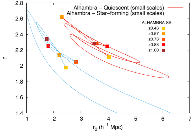
Figure 7. Parameters r_0 , \gamma obtained from the power-law fit to the projected correlation functions of our spectral segregated samples for the small scales ( r_p \leq 0.2 h^{-1} ). In red, the 1\sigma confidence regions of the quiescent galaxies fit and in blue, the 1\sigma confidence regions of the star-forming galaxies fit. For clarity, we show only the regions for the first and last redshift bin. Lines link the best-fit results for each sample across different redshift bins. The parameters and their 1-sigma variation have been calculated using the method described in Section 4.1
