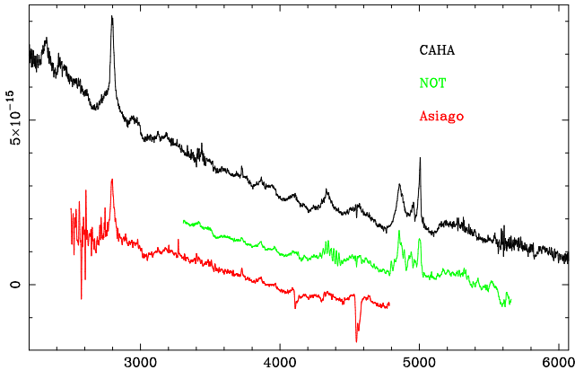
Figure 3. New spectra for 3C 57 covering MgII \lambda 2800 and H \beta in the rest frame. Abscissa is wavelength in Å and ordinate corresponds to specific flux in units of \text{erg s}^{-1} \text{cm}^{-2} \text{Å}^{-1} . NOT and Asiago spectra have been vertically displaced by -1 \times 10^{-15} \text{erg s}^{-1} \text{cm}^{-2} and -2 \times 10^{-15} \text{erg s}^{-1} \text{cm}^{-2} respectively for presentation.
