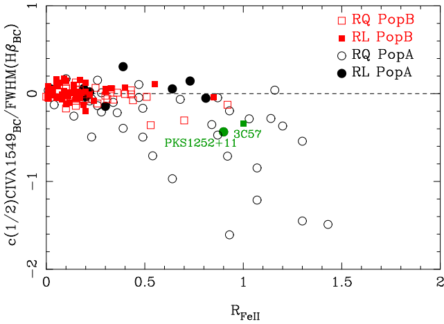
Figure 2. Location of 3C 57 and PKS 1252+11 in a 4DE1 UV-optical plane defined by normalized FWHM CIV \lambda 1549 vs. R_{FeII} . RL and RQ sources are marked as filled and open symbols respectively. Pop A sources are represented by black circles while Pop B by red squares.
