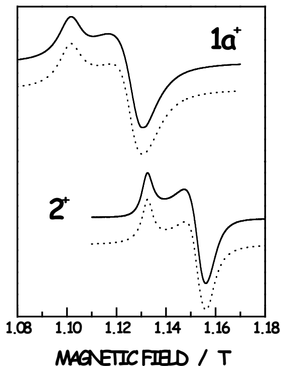
Figure 3. Q-band (34 GHz) EPR spectra of polycrystalline powdered sample of 1a^+ and 2^+ . Dotted lines correspond to calculated spectra with the parameters given in Table 3 (see text for details). These last ones have been shifted down a 25 % of their whole amplitude.
