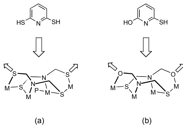
Scheme 1. Synthesis of tetranuclear complexes directed by 2,6-dimercaptopyridine (a) and 6-mercapto-pyridin-2-ol (b)
