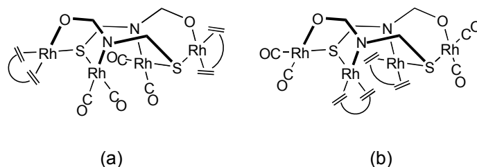
Figure 2. Possible C_2 isomers of compound [\text{Rh}_4(\mu\text{-PySO})_2(\text{cod})_2(\text{CO})_4] ( 5 ).
