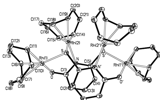
Figure 1. Molecular structure of compound [\text{Rh}_4(\mu\text{-PySO})_2(\text{cod})_4] ( 1 ). Selected bond distances (Å) and angles ( ^\circ ): Rh(1)-S 2.3890(10), Rh(1)-O 2.110(3), Rh(1)-C(6) 2.129(4), Rh(1)-C(7) 2.138(4), Rh(1)-C(10) 2.085(4), Rh(1)-C(11) 2.093(4), Rh(2)-S 2.3716(10), Rh(2)-N 2.093(3), Rh(2)-C(14) 2.139(4), Rh(2)-C(15) 2.134(4), Rh(2)-C(18) 2.137(4), Rh(2)-C(19) 2.142(4); S-Rh(1)-O 96.86(8), S-Rh(2)-N 86.97(9), S-Rh(1)-M(1) 176.65(11), S-Rh(2)-M(3) 170.53(13), S-Rh(1)-M(2) 90.07(12), S-Rh(2)-M(4) 94.4(6), O-Rh(1)-M(1) 85.26(13), N-Rh(2)-M(3) 91.28(14), O-Rh(1)-M(2) 170.59(13), N-Rh(2)-M(4) 178.6(8), Rh(1)-S-Rh(2) 83.52(3), Rh(1)-O-C(1) 128.2(2) (M labels represent the midpoints of the olefinic bonds).
