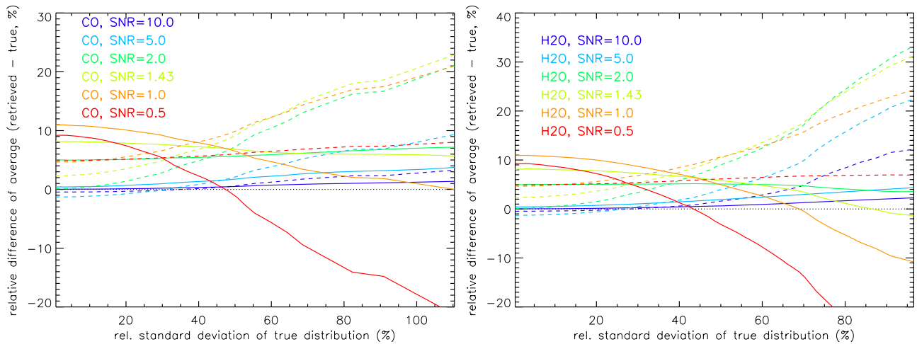
Fig. 8. Differences of retrieved and “true” zonal means (relative to the latter) versus local natural variability in terms of standard deviation for the CO (left) and H 2 O (right). Solid: linear averages, dashed: logarithmic averages. Simulations are performed with a modified maximum a posteriori ln(vmr)-retrieval simulations using a fixed constraint corresponding to climatological variance of 100 %. Results for signal to noise ratios of 10 (dark blue), 5 (light blue), 2 (dark green), 1.43 (light green), 1.0 (orange), and 0.5 (red) are shown. The resulting a priori contributions are 1 %, 3.8 %, 20 %, 33 %, 50 %, and 80 %, respectively.
