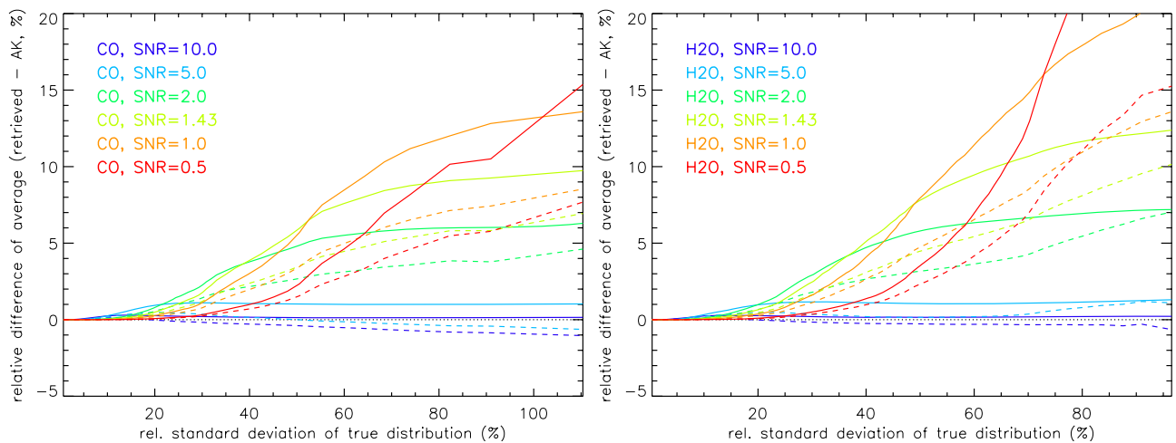
Fig. 7. Differences between the mean values and the mean “true” atmospheric state after application of the averaging kernel to the latter for CO (left) and H 2 O (right). Solid: linear averages, dashed: logarithmic averages. Results are shown for maximum a posteriori ln(vmr)-retrieval simulations with SNRs of 10 (dark blue), 5 (light blue), 2 (dark green), 1.43 (light green), 1.0 (orange), and 0.5 (red).
