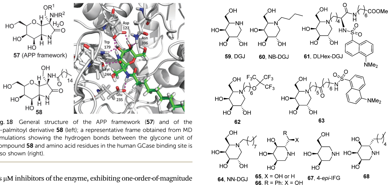
Fig. 19 Structures of iminosugar-type PCs for GM1.
