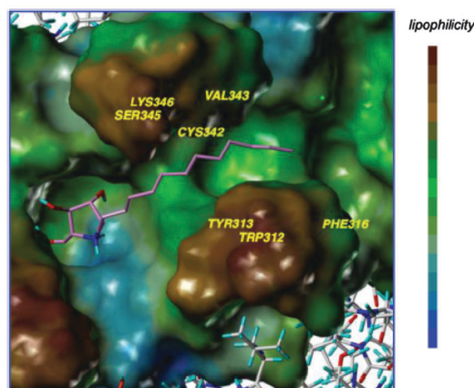
Fig. 9 Structure of \alpha -1-C-tridecyl-DAB ( 33 ) and its binding in the active site of GCase as obtained by docking.
