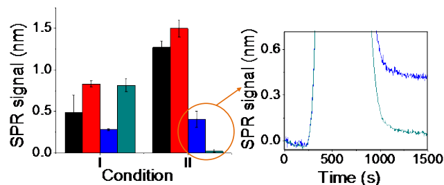
Fig. 1. SPR responses for the capture of 200 nM synthetic methylated (black) and 200 nM unmethylated (red) targets followed by their detection with 300 nM synthetic reading oligo (blue for methylated targets; aquamarine for unmethylated targets). The self-assembled monolayer of the thiolated capture probe was formed via (Condition I) ex-situ immobilisation of 1 \mu M thiolated DNA + 100 nM aqueous MCH and (Condition II) condition I + in-situ immobilisation of 1 mM aqueous MCH solution + capture of synthetic targets pre-treated with helper oligos. Right Panel: SPR sensorgrams of the reading oligos hybridized with methylated (blue) and unmethylated (aquamarine) targets. Each data point in left Panel represents the average of three separate trials ( n = 3 ), and error bars represent standard deviation of measurements within each experiments. Relative standard deviation was found to be <7.0\% ( n = 3 ).
