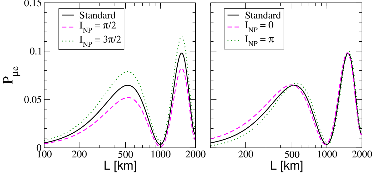
FIG. 3: Conversion probability for a fixed neutrino energy E_\nu = 1 GeV. The solid (black) curve shows the standard conversion probability, with \delta = -I_{123} = 3\pi/2 . The non-unitary case is illustrated for \alpha_{11} = 1 , \alpha_{22} = 0.9997 , and |\alpha_{21}| = 0.0264 . In the left panel, two values for the new CP phase parameter I_{NP} are considered: \pi/2 (dashed/magenta line) and 3\pi/2 (dotted/green line), while in the right panel we take I_{NP} = 0 (dashed/magenta line) and \pi (dotted/green line).
