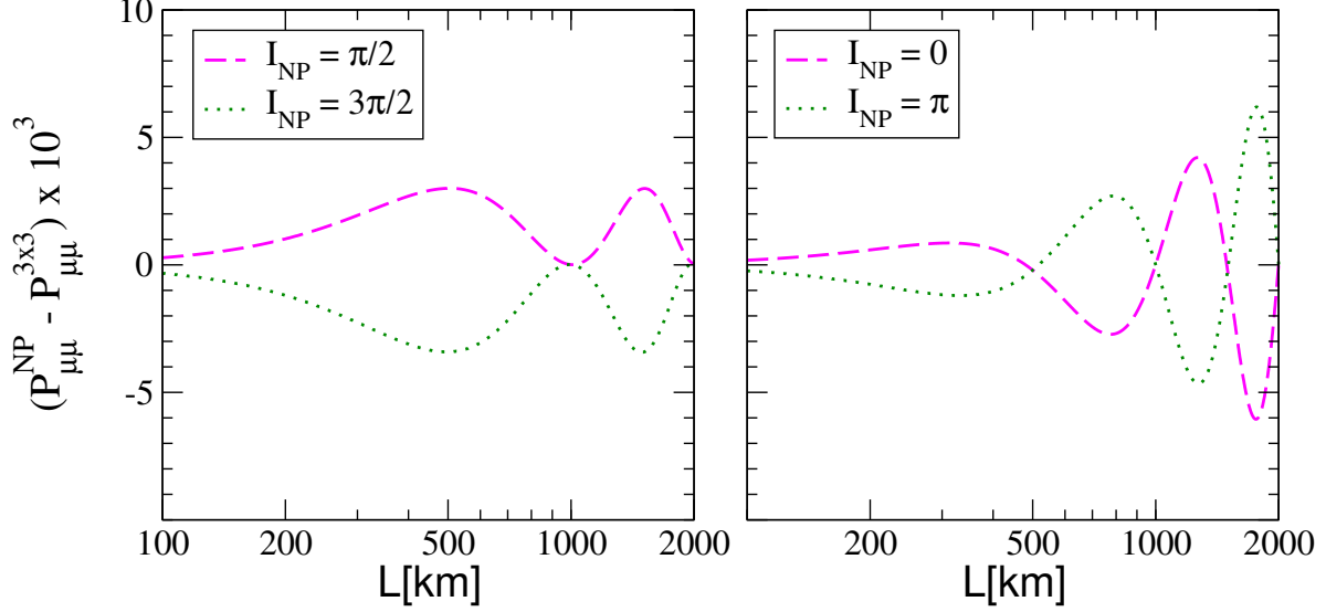
FIG. 4: Correction to the standard muon neutrino survival probability for different values of the new CP phase parameter I_{NP} , with the remaining parameters fixed as in Fig. 3.
